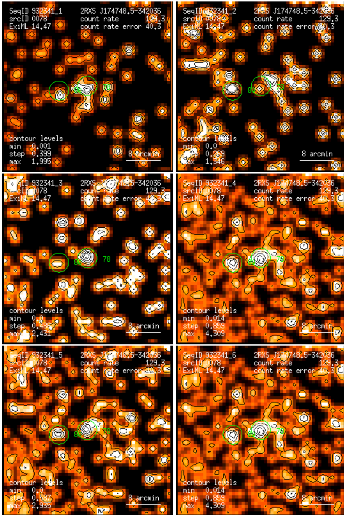
Figure 78: RASS 932341: detection 0078: band rate images, Gaussian filter: (1) PSPC channels 11 – 41, (2) 52 – 90, (3) 91 – 201, (4) 11 – 235, (5) 52 – 201, (6) 11 – 201. Broad band rates in counts/ks. Band rate contour levels in counts/ks/arcmin 2 .
