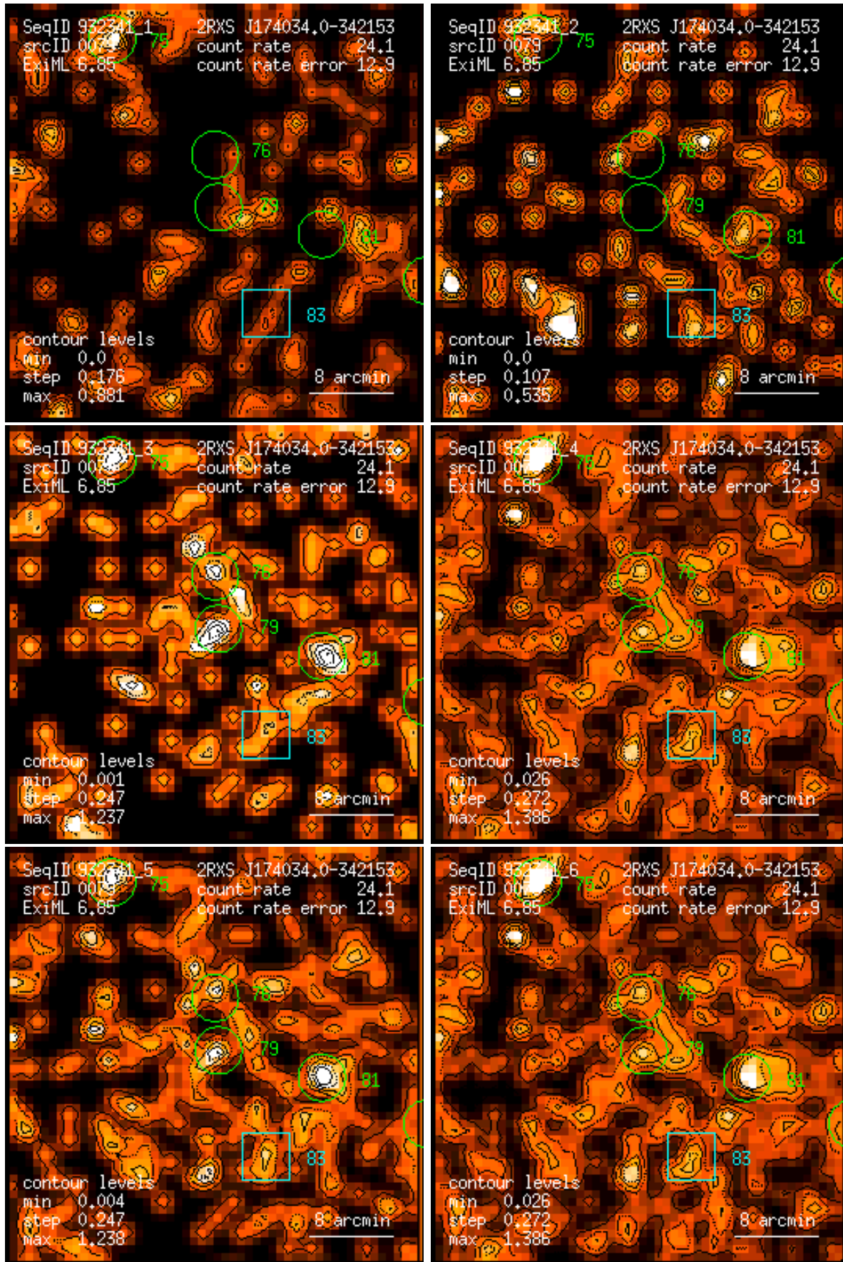
Figure 79: RASS 932341: detection 0079: band rate images, Gaussian filter: (1) PSPC channels 11 – 41, (2) 52 – 90, (3) 91 – 201, (4) 11 – 235, (5) 52 – 201, (6) 11 – 201. Broad band rates in counts/ks. Band rate contour levels in counts/ks/arcmin 2 .
