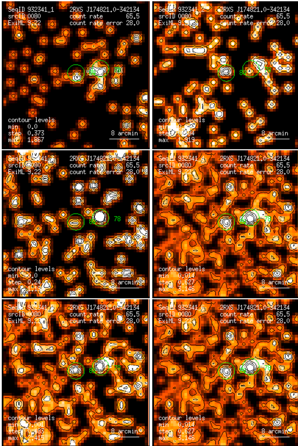
Figure 80: RASS 932341: detection 0080: band rate images, Gaussian filter: (1) PSPC channels 11 – 41, (2) 52 – 90, (3) 91 – 201, (4) 11 – 235, (5) 52 – 201, (6) 11 – 201. Broad band rates in counts/ks. Band rate contour levels in counts/ks/arcmin 2 .
