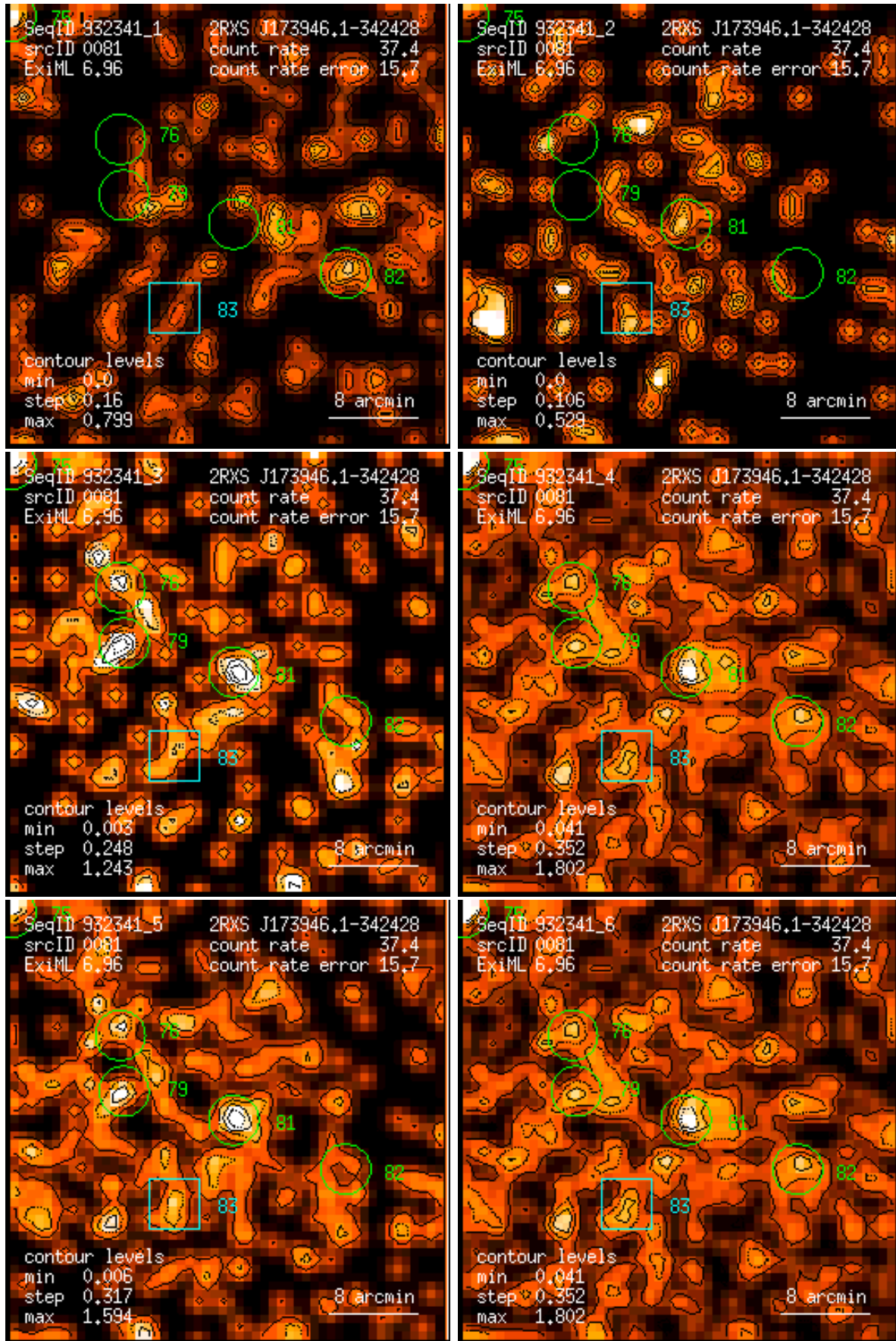
Figure 81: RASS 932341: detection 0081: band rate images, Gaussian filter: (1) PSPC channels 11 – 41, (2) 52 – 90, (3) 91 – 201, (4) 11 – 235, (5) 52 – 201, (6) 11 – 201. Broad band rates in counts/ks. Band rate contour levels in counts/ks/arcmin 2 .
