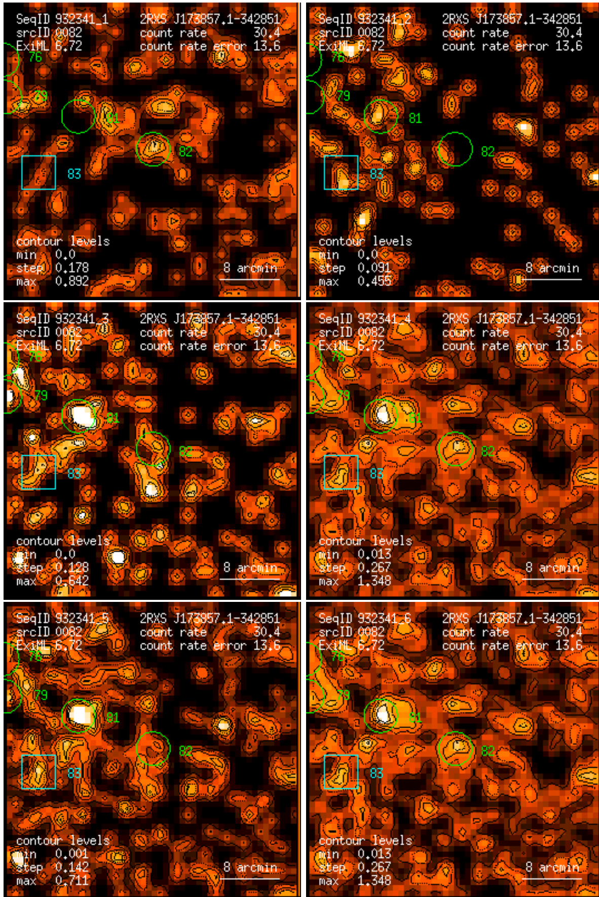
Figure 82: RASS 932341: detection 0082: band rate images, Gaussian filter: (1) PSPC channels 11 – 41, (2) 52 – 90, (3) 91 – 201, (4) 11 – 235, (5) 52 – 201, (6) 11 – 201. Broad band rates in counts/ks. Band rate contour levels in counts/ks/arcmin 2 .
