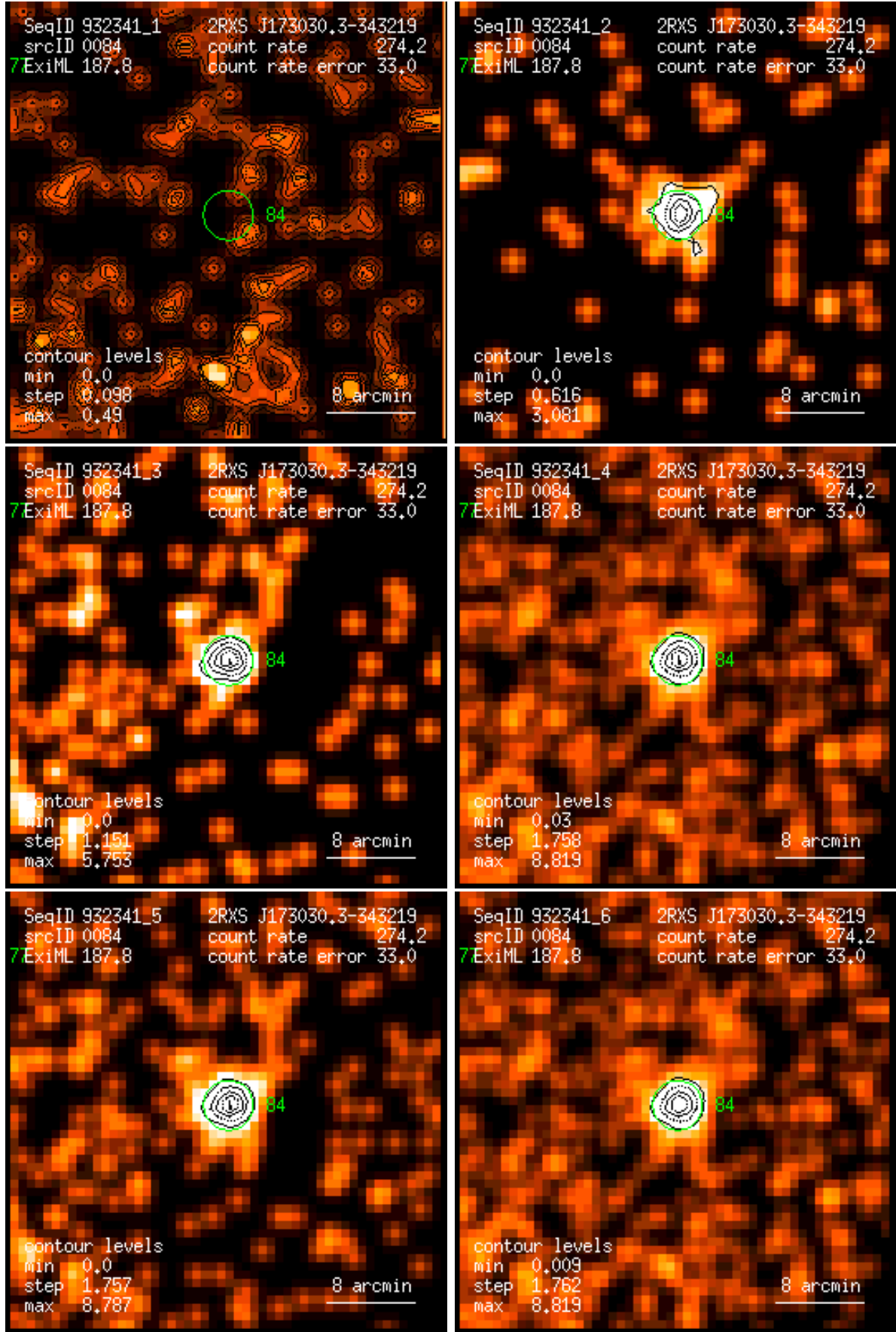
Figure 84: RASS 932341: detection 0084: band rate images, Gaussian filter: (1) PSPC channels 11 – 41, (2) 52 – 90, (3) 91 – 201, (4) 11 – 235, (5) 52 – 201, (6) 11 – 201. Broad band rates in counts/ks. Band rate contour levels in counts/ks/arcmin 2 .
