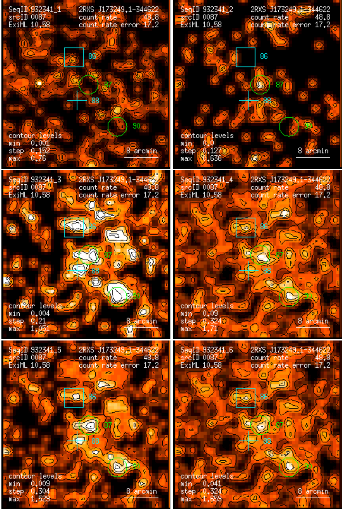
Figure 87: RASS 932341: detection 0087: band rate images, Gaussian filter: (1) PSPC channels 11 – 41, (2) 52 – 90, (3) 91 – 201, (4) 11 – 235, (5) 52 – 201, (6) 11 – 201. Broad band rates in counts/ks. Band rate contour levels in counts/ks/arcmin 2 .
