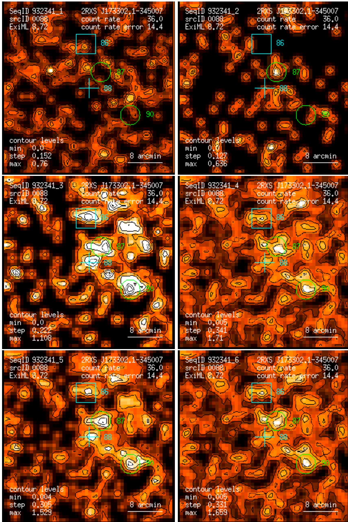
Figure 88: RASS 932341: detection 0088: band rate images, Gaussian filter: (1) PSPC channels 11 – 41, (2) 52 – 90, (3) 91 – 201, (4) 11 – 235, (5) 52 – 201, (6) 11 – 201. Broad band rates in counts/ks. Band rate contour levels in counts/ks/arcmin 2 .
