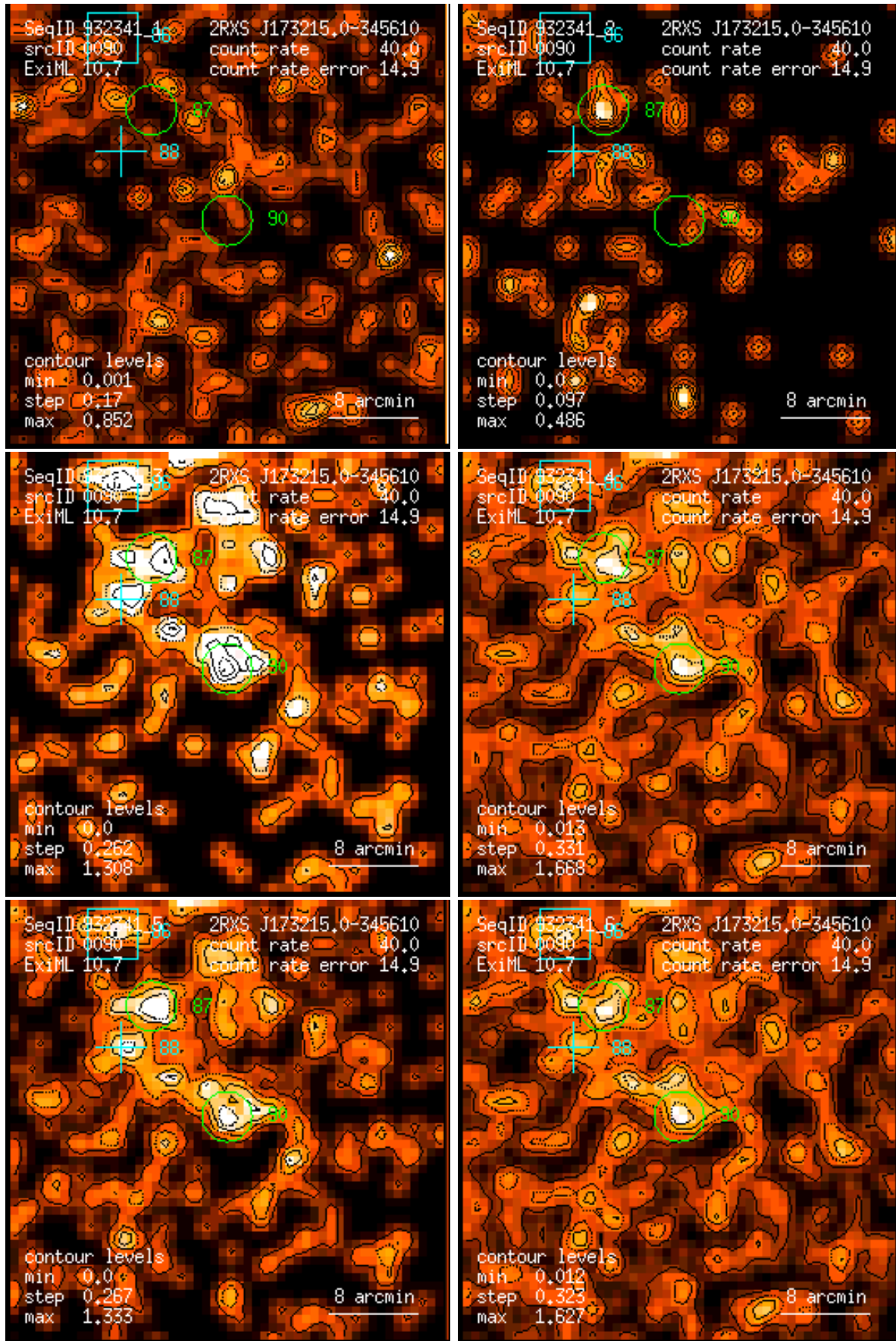
Figure 90: RASS 932341: detection 0090: band rate images, Gaussian filter: (1) PSPC channels 11 – 41, (2) 52 – 90, (3) 91 – 201, (4) 11 – 235, (5) 52 – 201, (6) 11 – 201. Broad band rates in counts/ks. Band rate contour levels in counts/ks/arcmin 2 .
