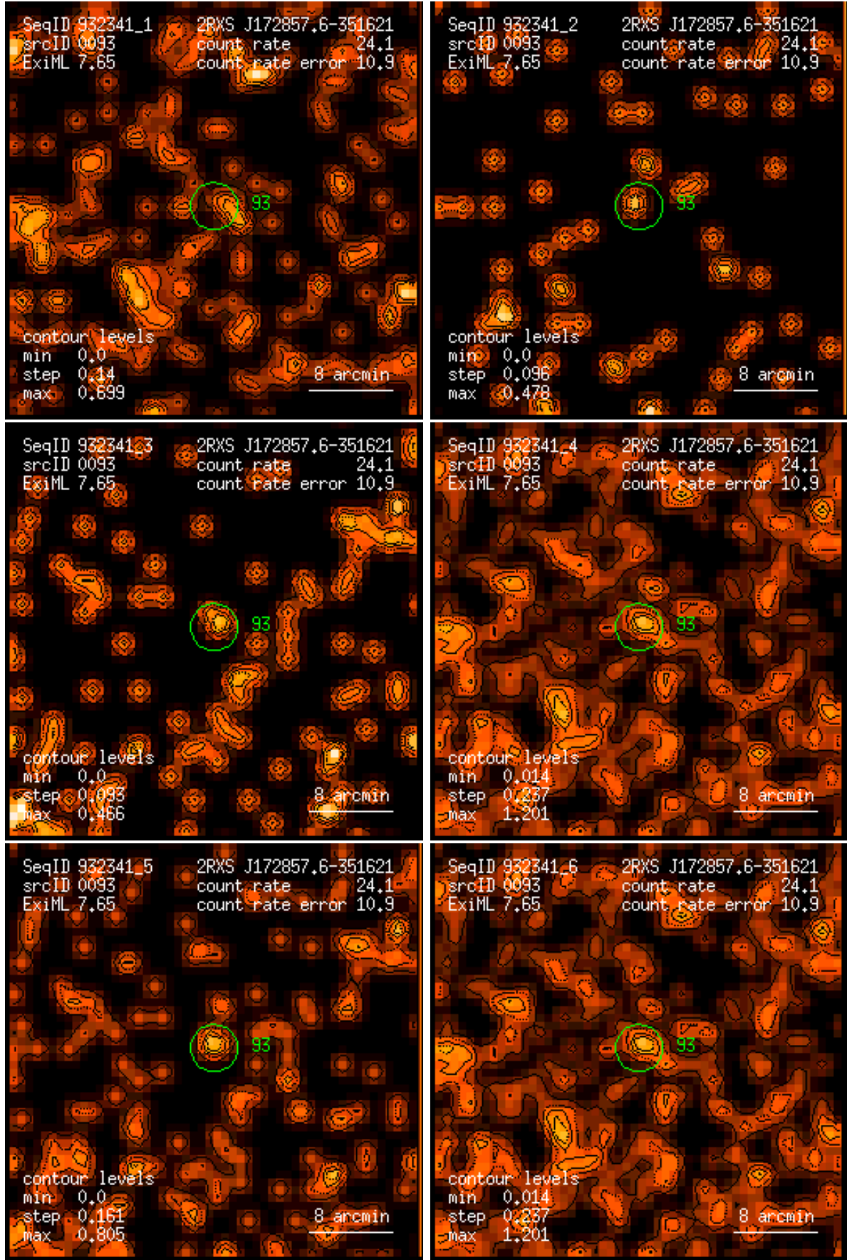
Figure 93: RASS 932341: detection 0093: band rate images, Gaussian filter: (1) PSPC channels 11 – 41, (2) 52 – 90, (3) 91 – 201, (4) 11 – 235, (5) 52 – 201, (6) 11 – 201. Broad band rates in counts/ks. Band rate contour levels in counts/ks/arcmin 2 .
