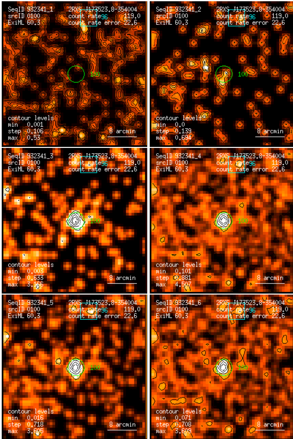
Figure 100: RASS 932341: detection 0100: band rate images, Gaussian filter: (1) PSPC channels 11 – 41, (2) 52 – 90, (3) 91 – 201, (4) 11 – 235, (5) 52 – 201, (6) 11 – 201. Broad band rates in counts/ks. Band rate contour levels in counts/ks/arcmin 2 .
