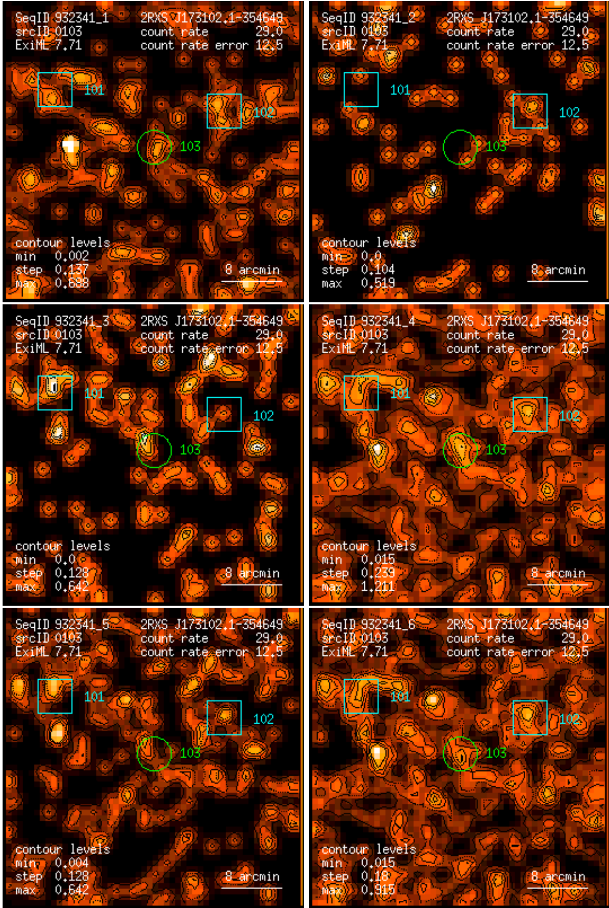
Figure 103: RASS 932341: detection 0103: band rate images, Gaussian filter: (1) PSPC channels 11 – 41, (2) 52 – 90, (3) 91 – 201, (4) 11 – 235, (5) 52 – 201, (6) 11 – 201. Broad band rates in counts/ks. Band rate contour levels in counts/ks/arcmin 2 .
