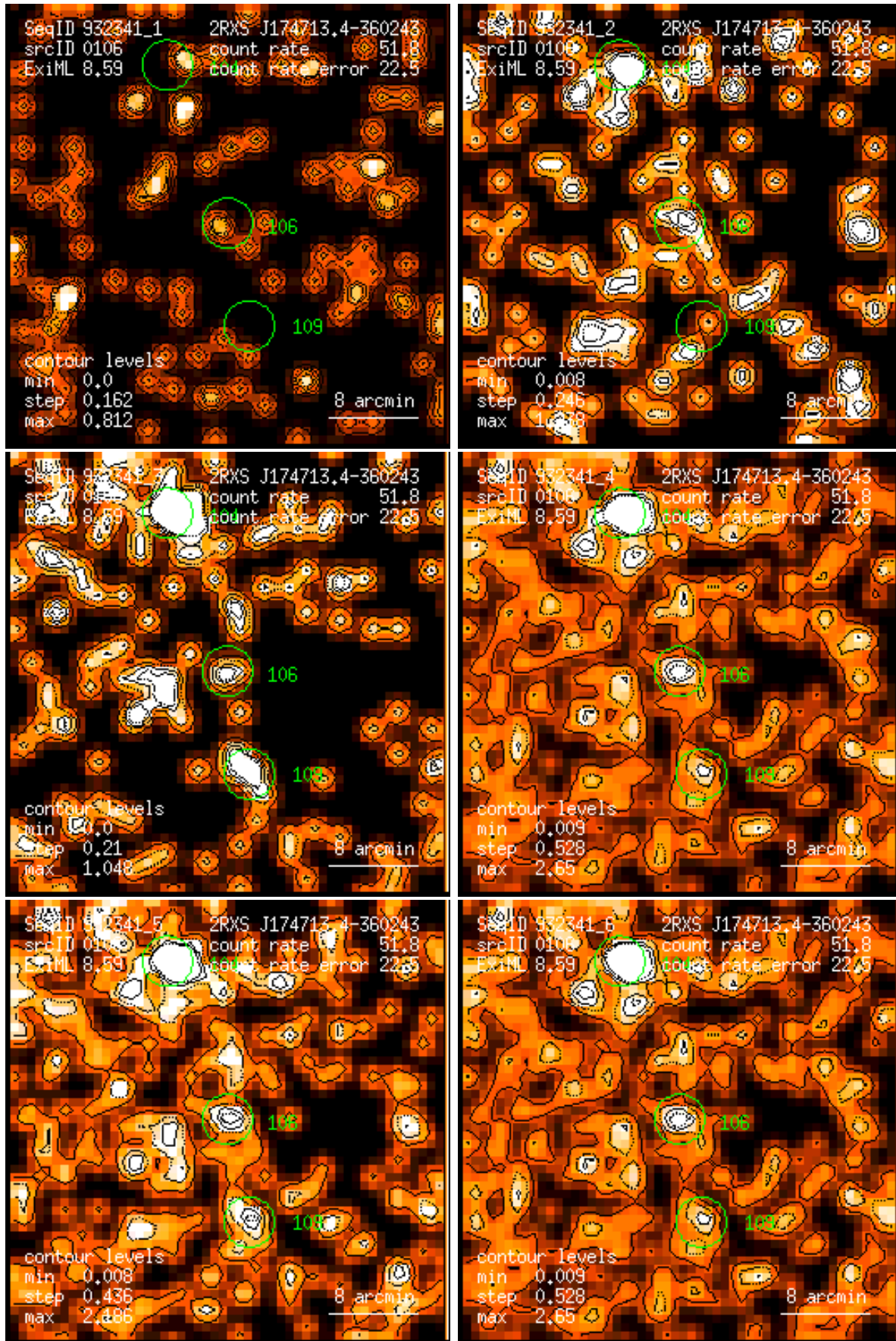
Figure 106: RASS 932341: detection 0106: band rate images, Gaussian filter: (1) PSCC channels 11 – 41, (2) 52 – 90, (3) 91 – 201, (4) 11 – 235, (5) 52 – 201, (6) 11 – 201. Broad band rates in counts/ks. Band rate contour levels in counts/ks/arcmin 2 .
