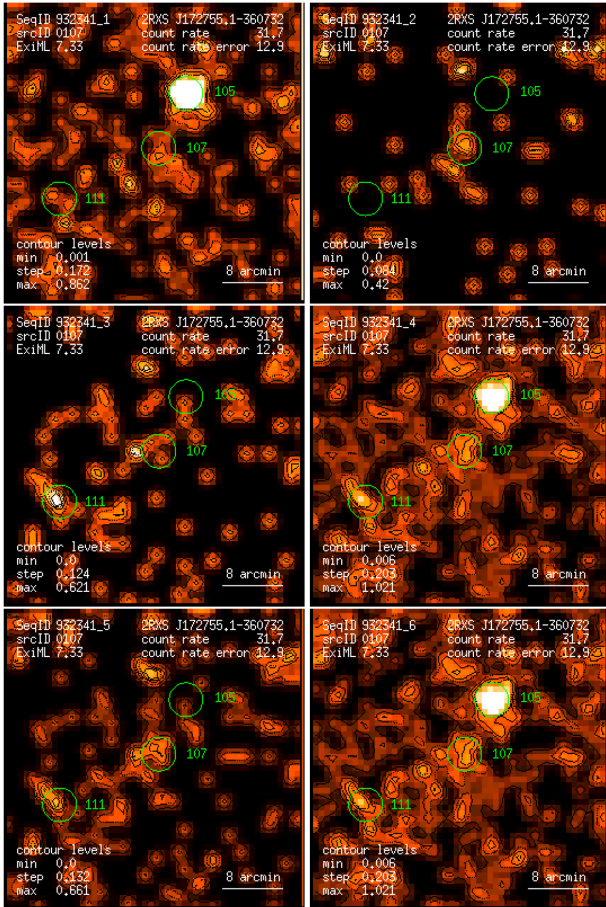
Figure 107: RASS 932341: detection 0107: band rate images, Gaussian filter: (1) PSPC channels 11 – 41, (2) 52 – 90, (3) 91 – 201, (4) 11 – 235, (5) 52 – 201, (6) 11 – 201. Broad band rates in counts/ks. Band rate contour levels in counts/ks/arcmin 2 .
