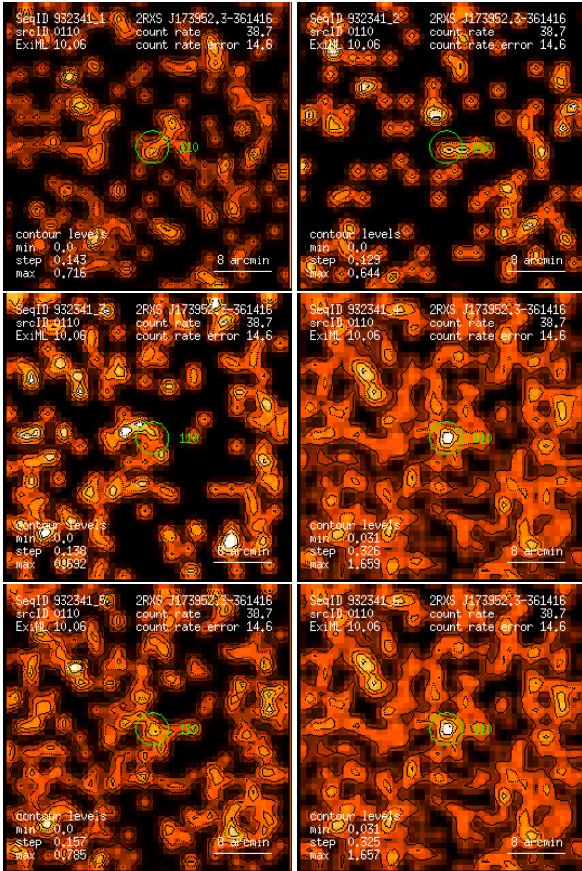
Figure 110: RASS 932341: detection 0110: band rate images, Gaussian filter: (1) PSPC channels 11 – 41, (2) 52 – 90, (3) 91 – 201, (4) 11 – 235, (5) 52 – 201, (6) 11 – 201. Broad band rates in counts/ks. Band rate contour levels in counts/ks/arcmin 2 .
