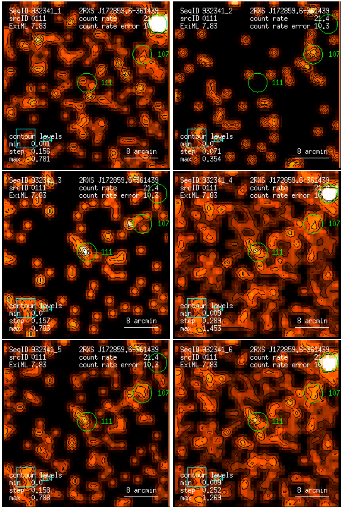
Figure 111: RASS 932341: detection 0111: band rate images, Gaussian filter: (1) PSPC channels 11 – 41, (2) 52 – 90, (3) 91 – 201, (4) 11 – 235, (5) 52 – 201, (6) 11 – 201. Broad band rates in counts/ks. Band rate contour levels in counts/ks/arcmin 2 .
