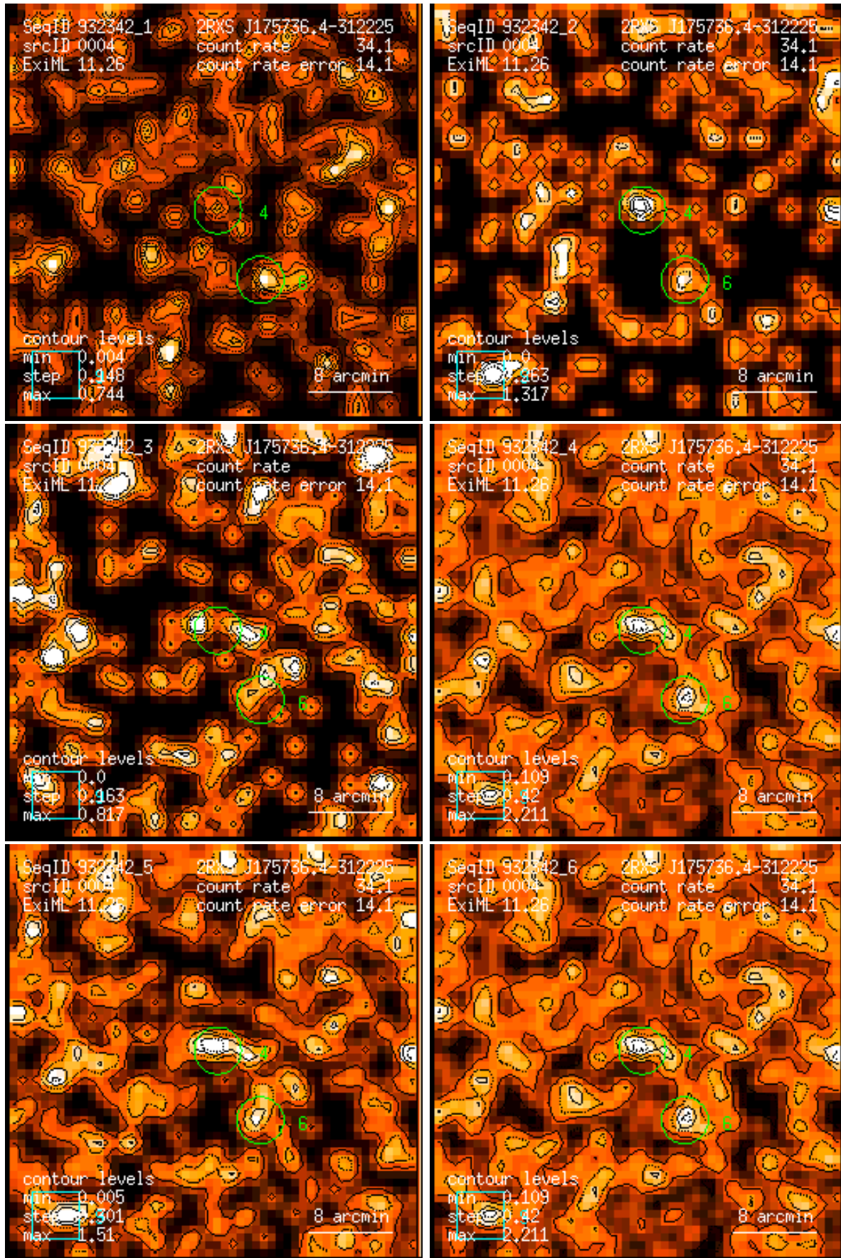
Figure 4: RASS 932342: detection 0004: band rate images, Gaussian filter: (1) PSPC channels 11 – 41, (2) 52 – 90, (3) 91 – 201, (4) 11 – 235, (5) 52 – 201, (6) 11 – 201. Broad band rates in counts/ks. Band rate contour levels in counts/ks/arcmin 2 .
