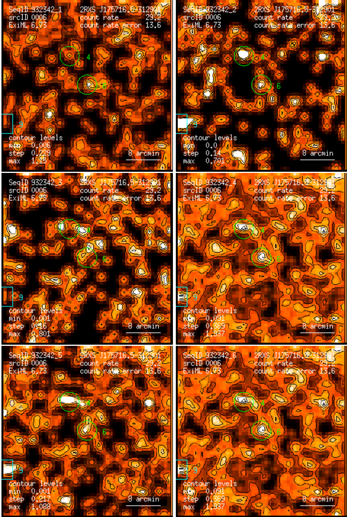
Figure 6: RASS 932342: detection 0006: band rate images, Gaussian filter: (1) PSPC channels 11 – 41, (2) 52 – 90, (3) 91 – 201, (4) 11 – 235, (5) 52 – 201, (6) 11 – 201. Broad band rates in counts/ks. Band rate contour levels in counts/ks/arcmin 2 .
