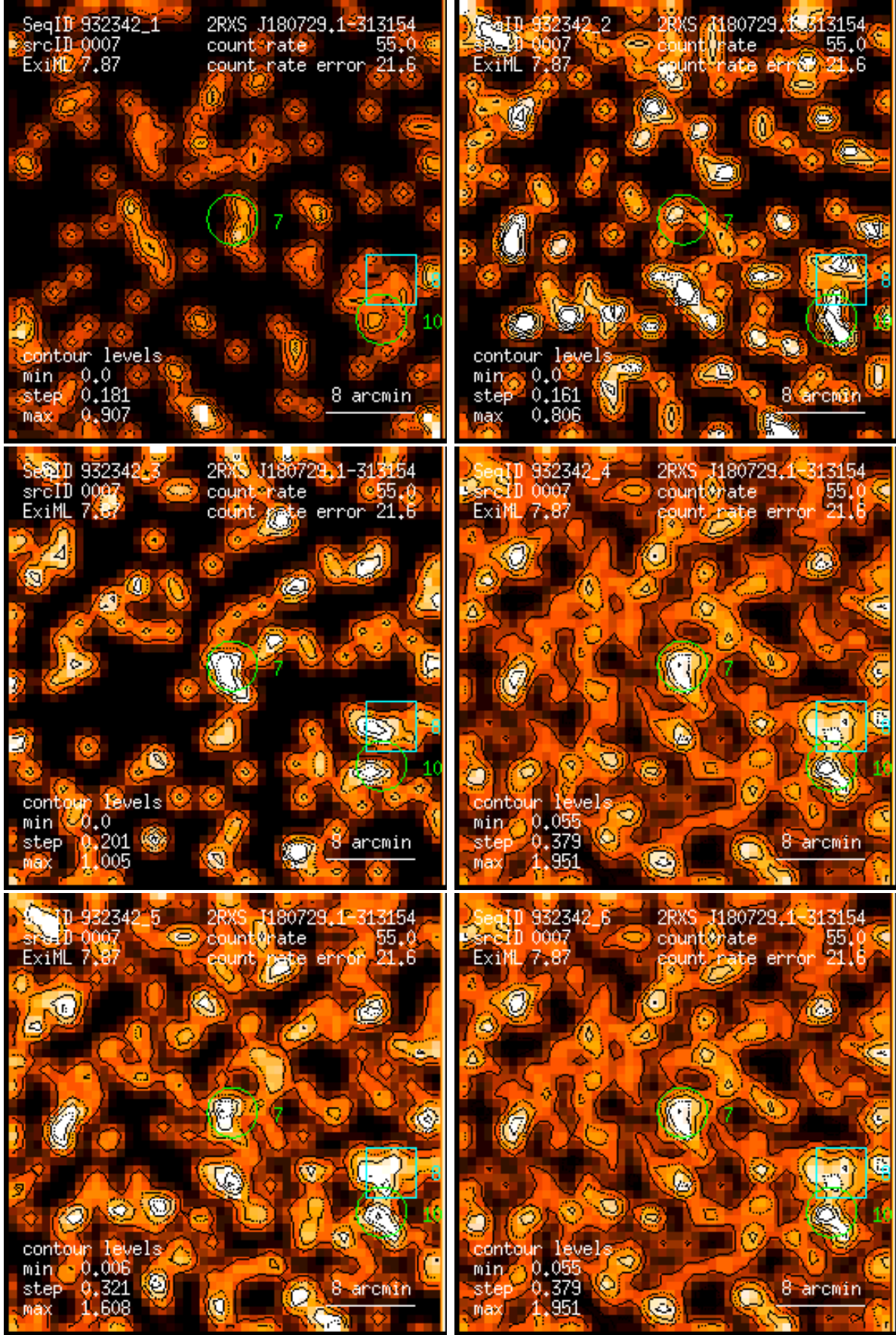
Figure 7: RASS 932342: detection 0007: band rate images, Gaussian filter: (1) PSPC channels 11 – 41, (2) 52 – 90, (3) 91 – 201, (4) 11 – 235, (5) 52 – 201, (6) 11 – 201. Broad band rates in counts/ks. Band rate contour levels in counts/ks/arcmin 2 .
