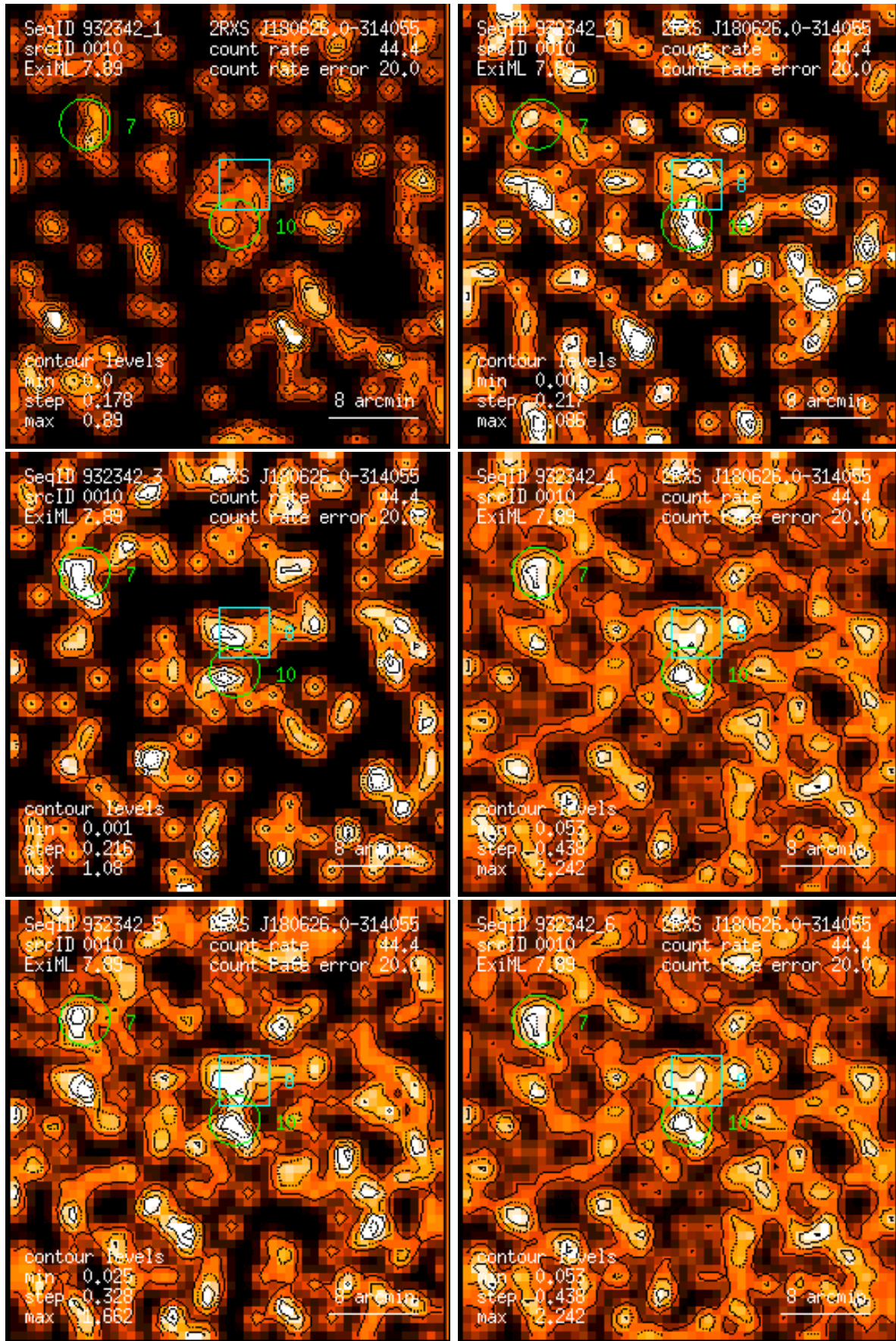
Figure 10: RASS 932342: detection 0010: band rate images, Gaussian filter: (1) PSPC channels 11 – 41, (2) 52 – 90, (3) 91 – 201, (4) 11 – 235, (5) 52 – 201, (6) 11 – 201. Broad band rates in counts/ks. Band rate contour levels in counts/ks/arcmin 2 .
