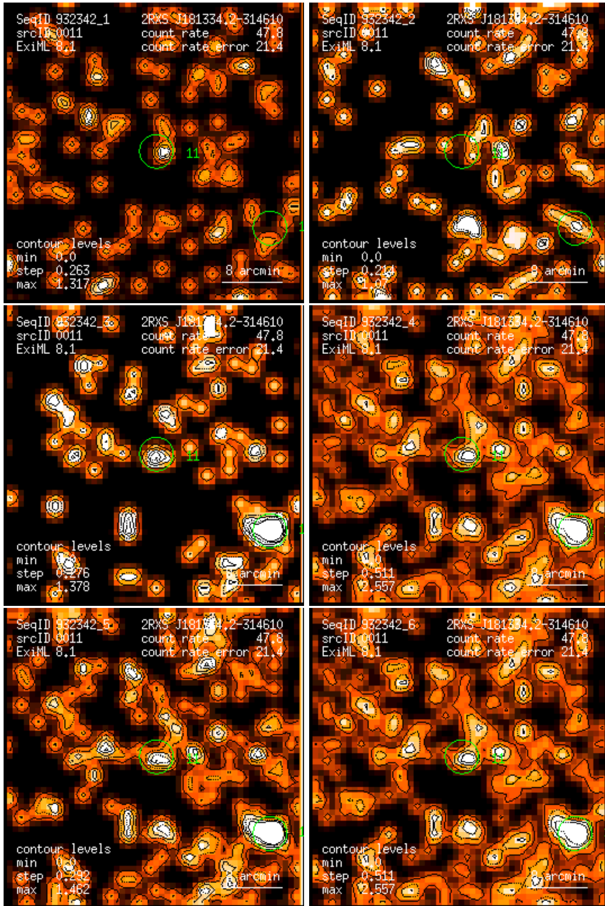
Figure 11: RASS 932342: detection 0011: band rate images, Gaussian filter: (1) PSPC channels 11 – 41, (2) 52 – 90, (3) 91 – 201, (4) 11 – 235, (5) 52 – 201, (6) 11 – 201. Broad band rates in counts/ks. Band rate contour levels in counts/ks/arcmin 2 .
