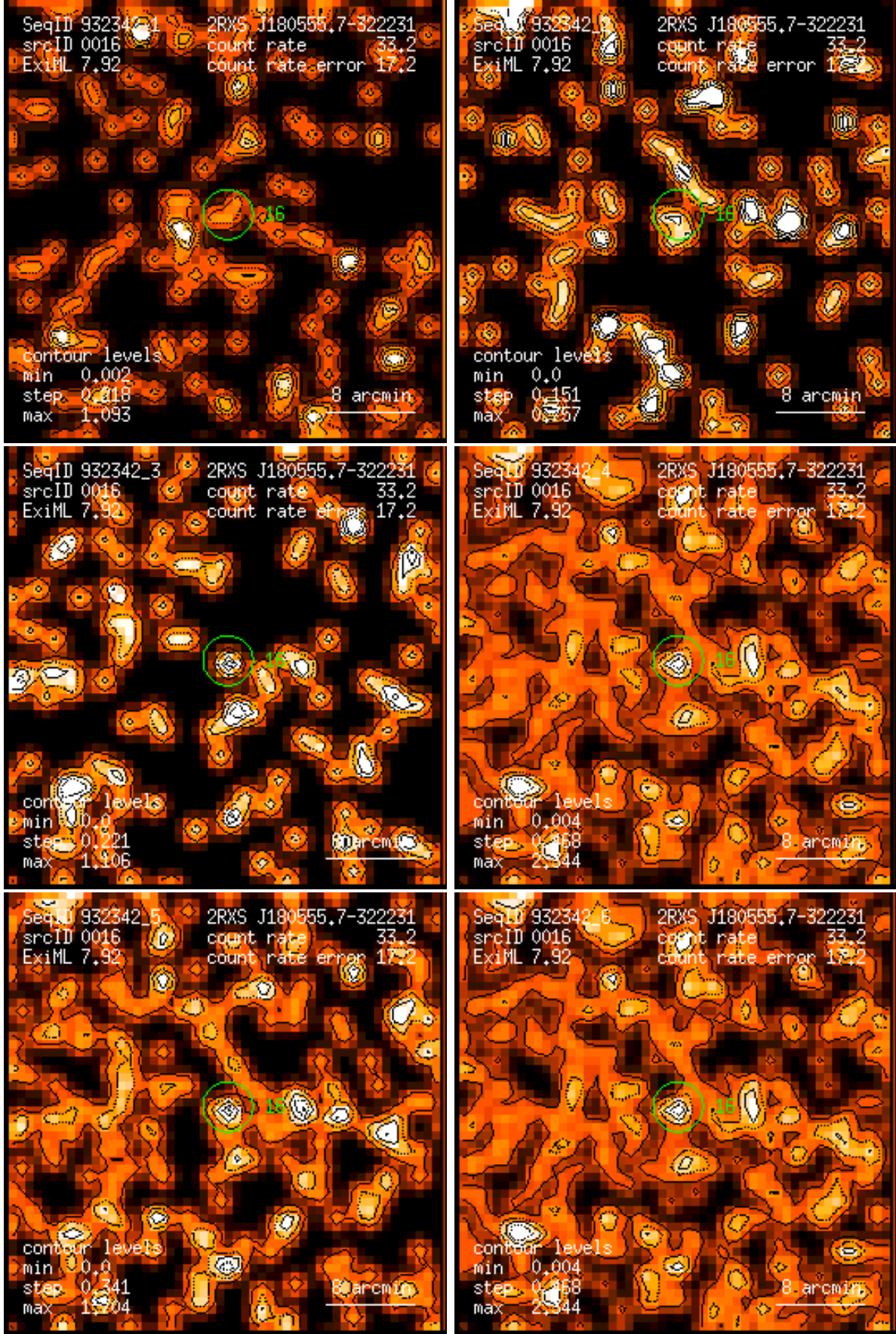
Figure 16: RASS 932342: detection 0016: band rate images, Gaussian filter: (1) PSPC channels 11 – 41, (2) 52 – 90, (3) 91 – 201, (4) 11 – 235, (5) 52 – 201, (6) 11 – 201. Broad band rates in counts/ks. Band rate contour levels in counts/ks/arcmin 2 .
