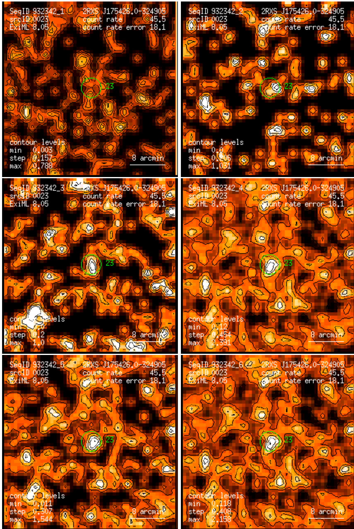
Figure 23: RASS 932342: detection 0023: band rate images, Gaussian filter: (1) PSPC channels 11 – 41, (2) 52 – 90, (3) 91 – 201, (4) 11 – 235, (5) 52 – 201, (6) 11 – 201. Broad band rates in counts/ks. Band rate contour levels in counts/ks/arcmin 2 .
