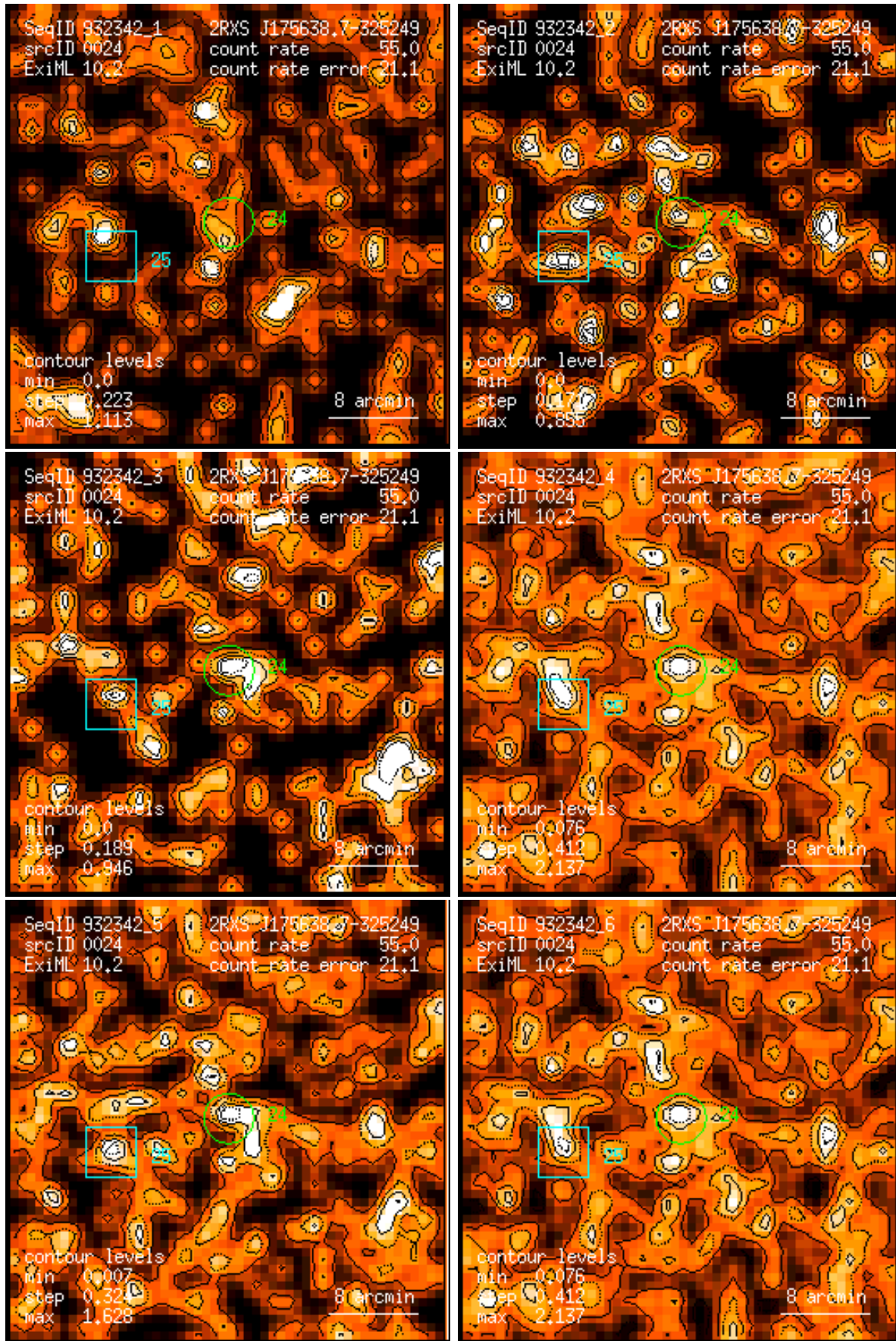
Figure 24: RASS 932342: detection 0024: band rate images, Gaussian filter: (1) PSPC channels 11 – 41, (2) 52 – 90, (3) 91 – 201, (4) 11 – 235, (5) 52 – 201, (6) 11 – 201. Broad band rates in counts/ks. Band rate contour levels in counts/ks/arcmin 2 .
