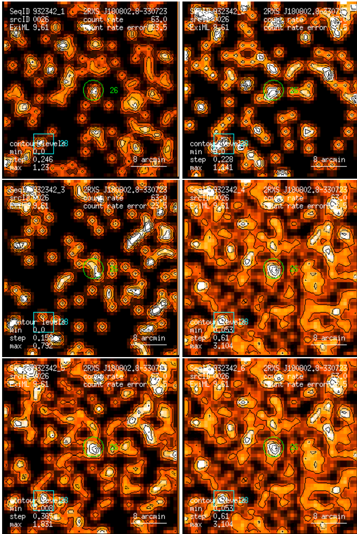
Figure 26: RASS 932342: detection 0026: band rate images, Gaussian filter: (1) PSPC channels 11 – 41, (2) 52 – 90, (3) 91 – 201, (4) 11 – 235, (5) 52 – 201, (6) 11 – 201. Broad band rates in counts/ks. Band rate contour levels in counts/ks/arcmin 2 .
