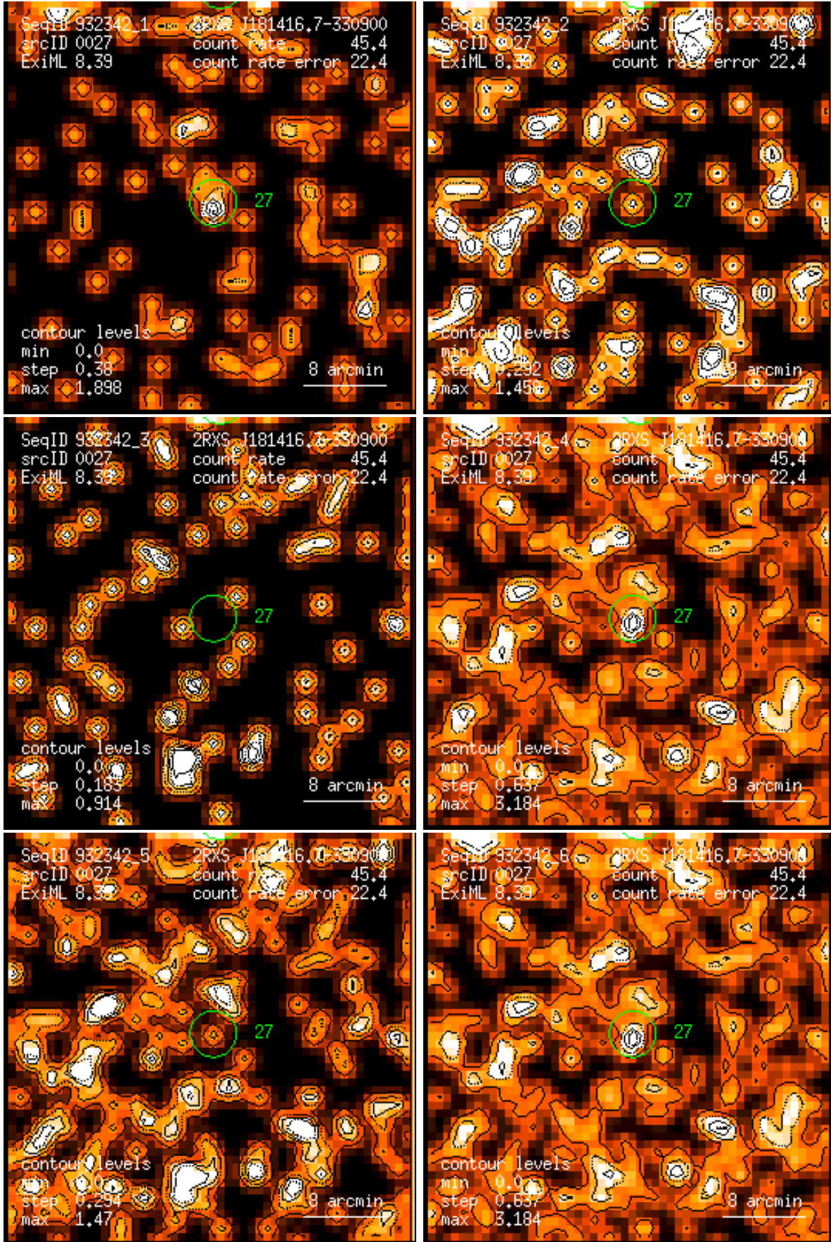
Figure 27: RASS 932342: detection 0027: band rate images, Gaussian filter: (1) PSPC channels 11 – 41, (2) 52 – 90, (3) 91 – 201, (4) 11 – 235, (5) 52 – 201, (6) 11 – 201. Broad band rates in counts/ks. Band rate contour levels in counts/ks/arcmin 2 .
