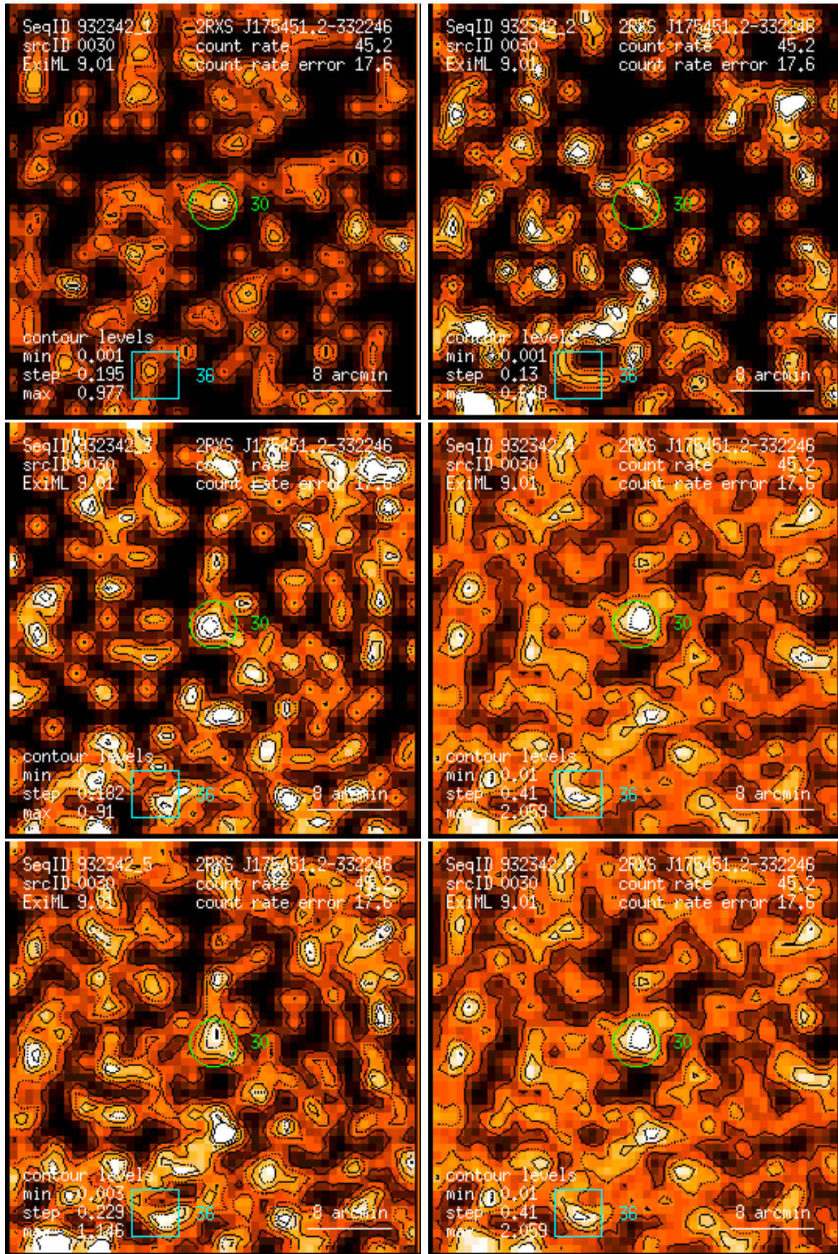
Figure 30: RASS 932342: detection 0030: band rate images, Gaussian filter: (1) PSPC channels 11 – 41, (2) 52 – 90, (3) 91 – 201, (4) 11 – 235, (5) 52 – 201, (6) 11 – 201. Broad band rates in counts/ks. Band rate contour levels in counts/ks/arcmin 2 .
