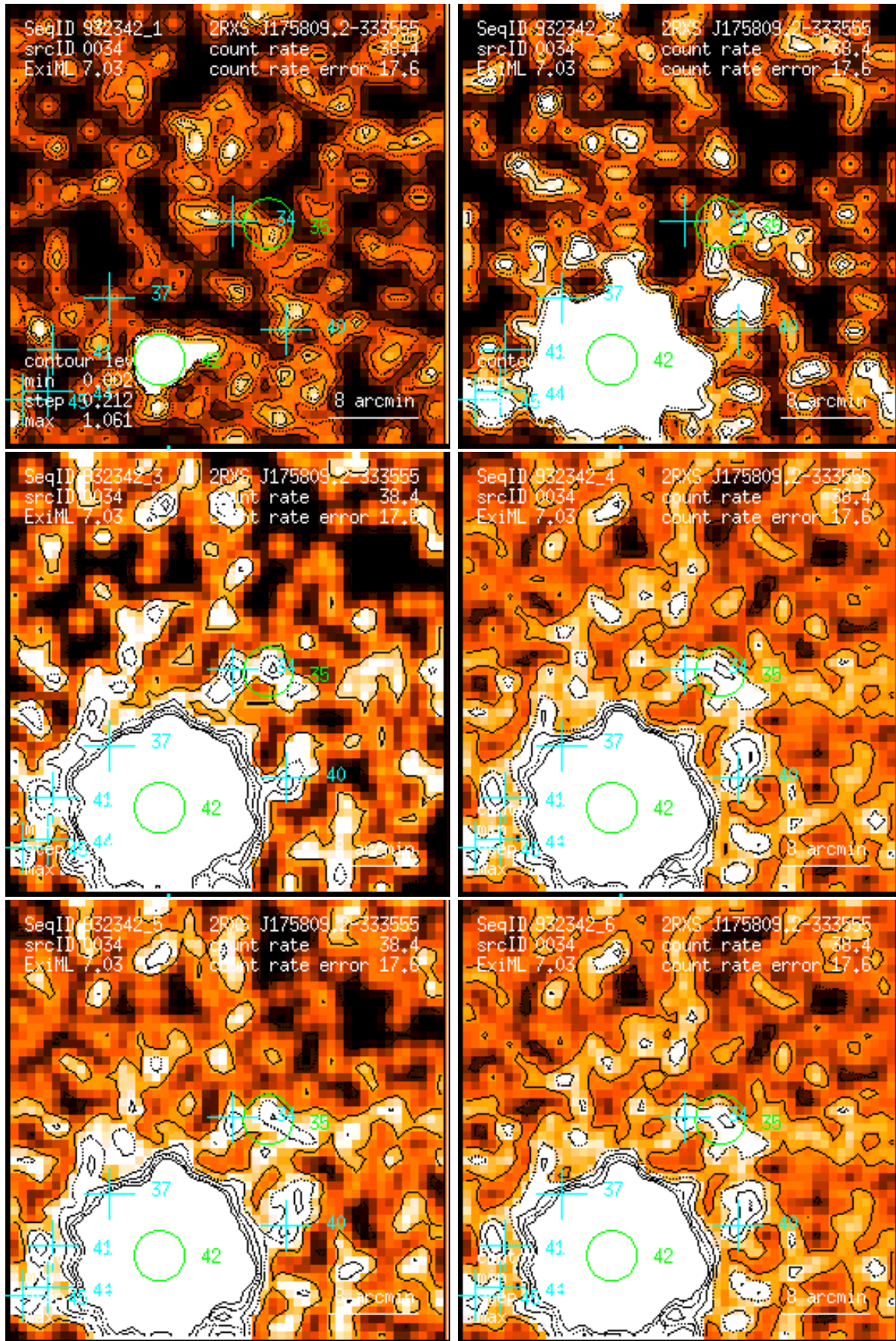
Figure 34: RASS 932342: detection 0034: band rate images, Gaussian filter: (1) PSPC channels 11 – 41, (2) 52 – 90, (3) 91 – 201, (4) 11 – 235, (5) 52 – 201, (6) 11 – 201. Broad band rates in counts/ks. Band rate contour levels in counts/ks/arcmin 2 .
