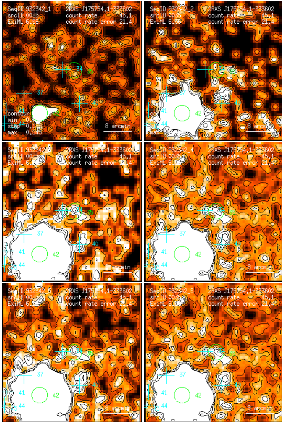
Figure 35: RASS 932342: detection 0035: band rate images, Gaussian filter: (1) PSPC channels 11 – 41, (2) 52 – 90, (3) 91 – 201, (4) 11 – 235, (5) 52 – 201, (6) 11 – 201. Broad band rates in counts/ks. Band rate contour levels in counts/ks/arcmin 2 .
