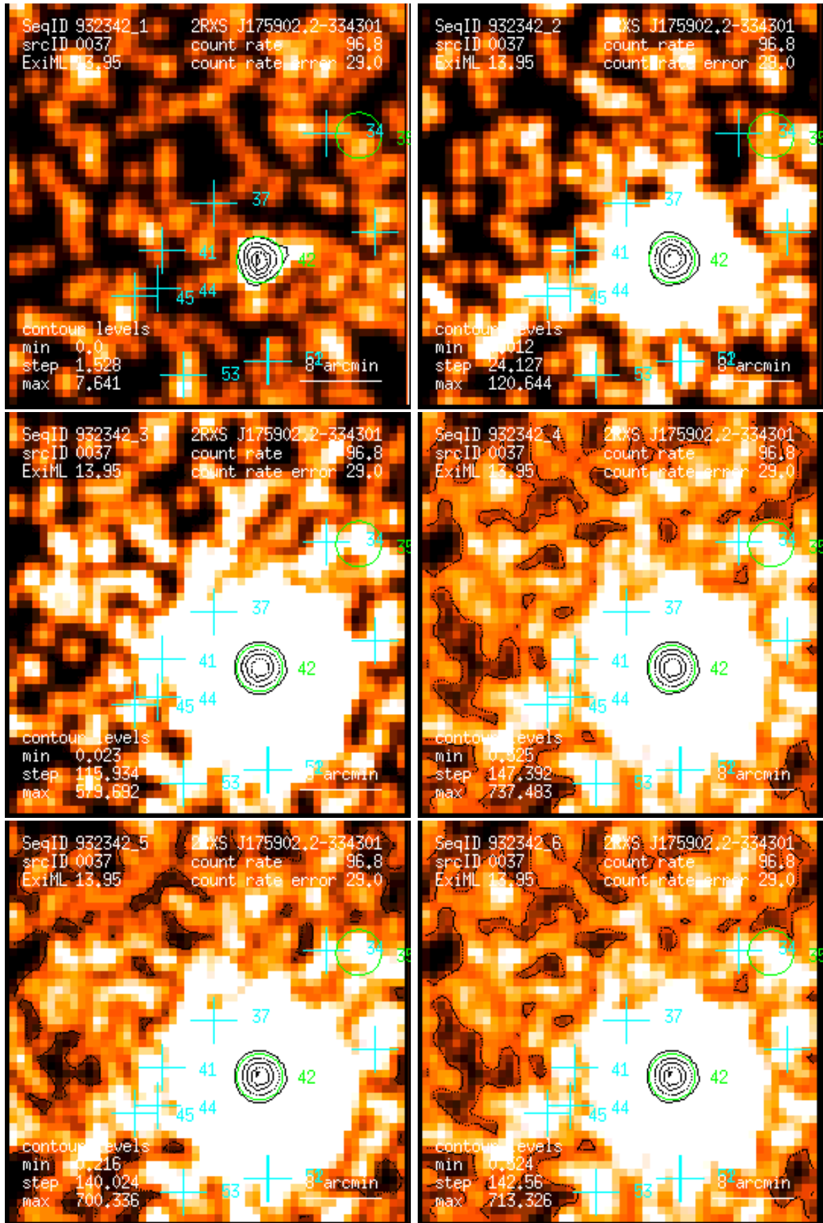
Figure 37: RASS 932342: detection 0037: band rate images, Gaussian filter: (1) PSPC channels 11 – 41, (2) 52 – 90, (3) 91 – 201, (4) 11 – 235, (5) 52 – 201, (6) 11 – 201. Broad band rates in counts/ks. Band rate contour levels in counts/ks/arcmin 2 .
