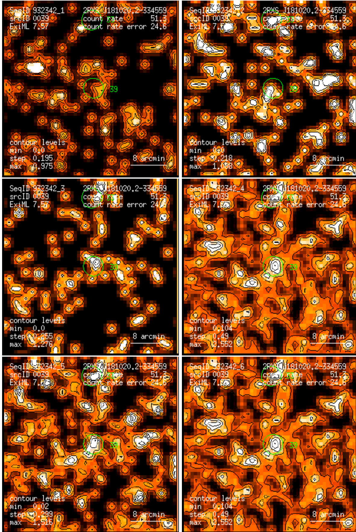
Figure 39: RASS 932342: detection 0039: band rate images, Gaussian filter: (1) PSPC channels 11 – 41, (2) 52 – 90, (3) 91 – 201, (4) 11 – 235, (5) 52 – 201, (6) 11 – 201. Broad band rates in counts/ks. Band rate contour levels in counts/ks/arcmin 2 .
