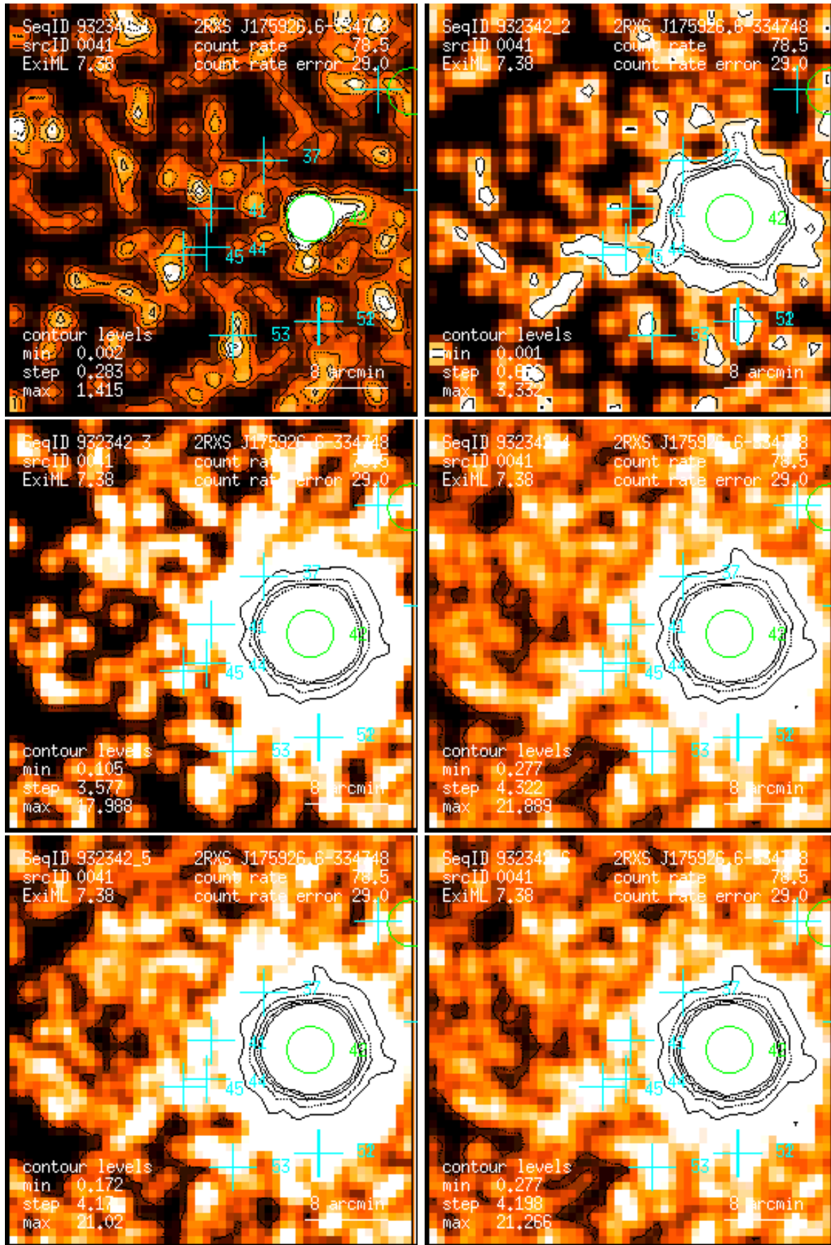
Figure 41: RASS 932342: detection 0041: band rate images, Gaussian filter: (1) PSPC channels 11 – 41, (2) 52 – 90, (3) 91 – 201, (4) 11 – 235, (5) 52 – 201, (6) 11 – 201. Broad band rates in counts/ks. Band rate contour levels in counts/ks/arcmin 2 .
