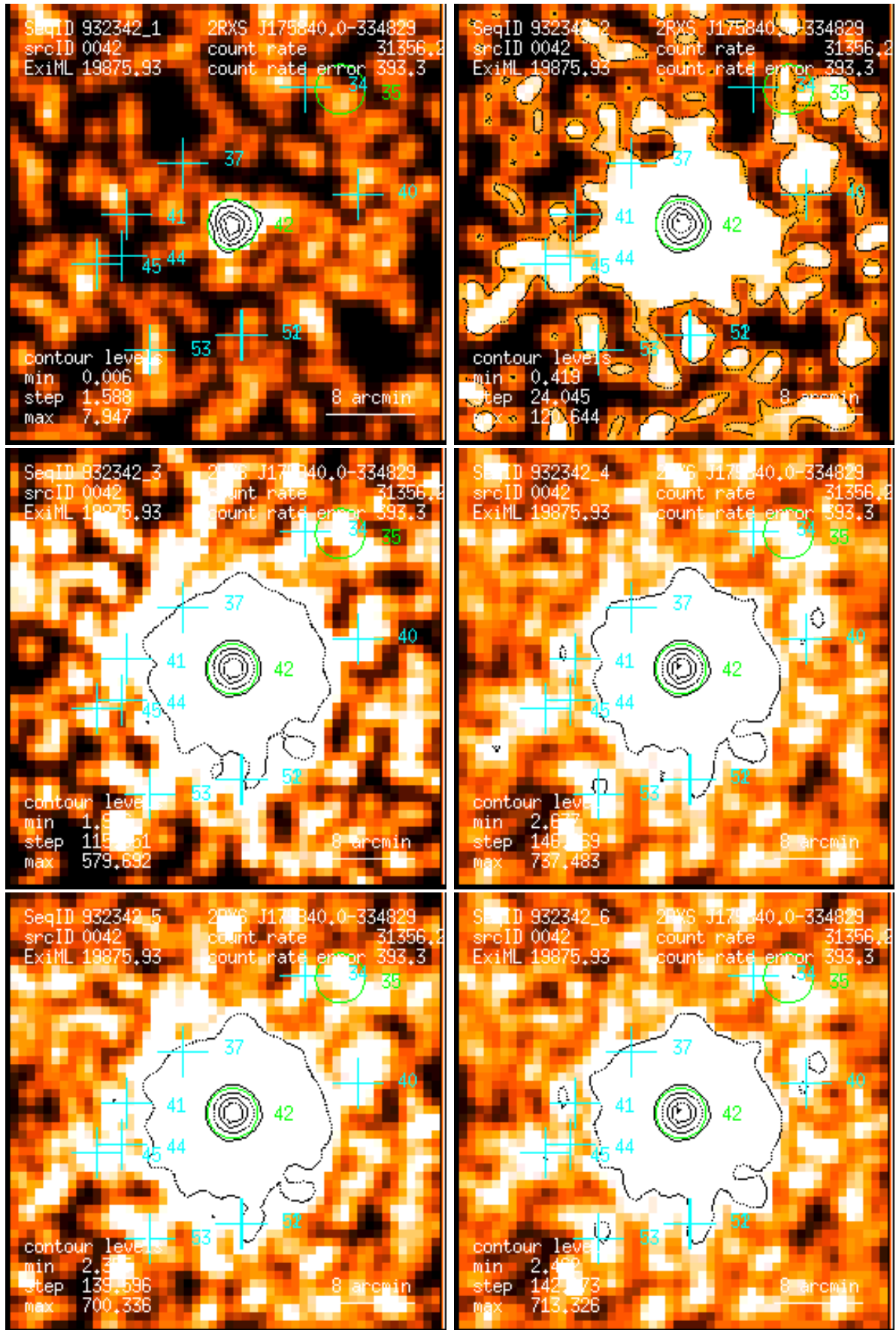
Figure 42: RASS 932342: detection 0042: band rate images, Gaussian filter: (1) PSPC channels 11 – 41, (2) 52 – 90, (3) 91 – 201, (4) 11 – 235, (5) 52 – 201, (6) 11 – 201. Broad band rates in counts/ks. Band rate contour levels in counts/ks/arcmin 2 .
