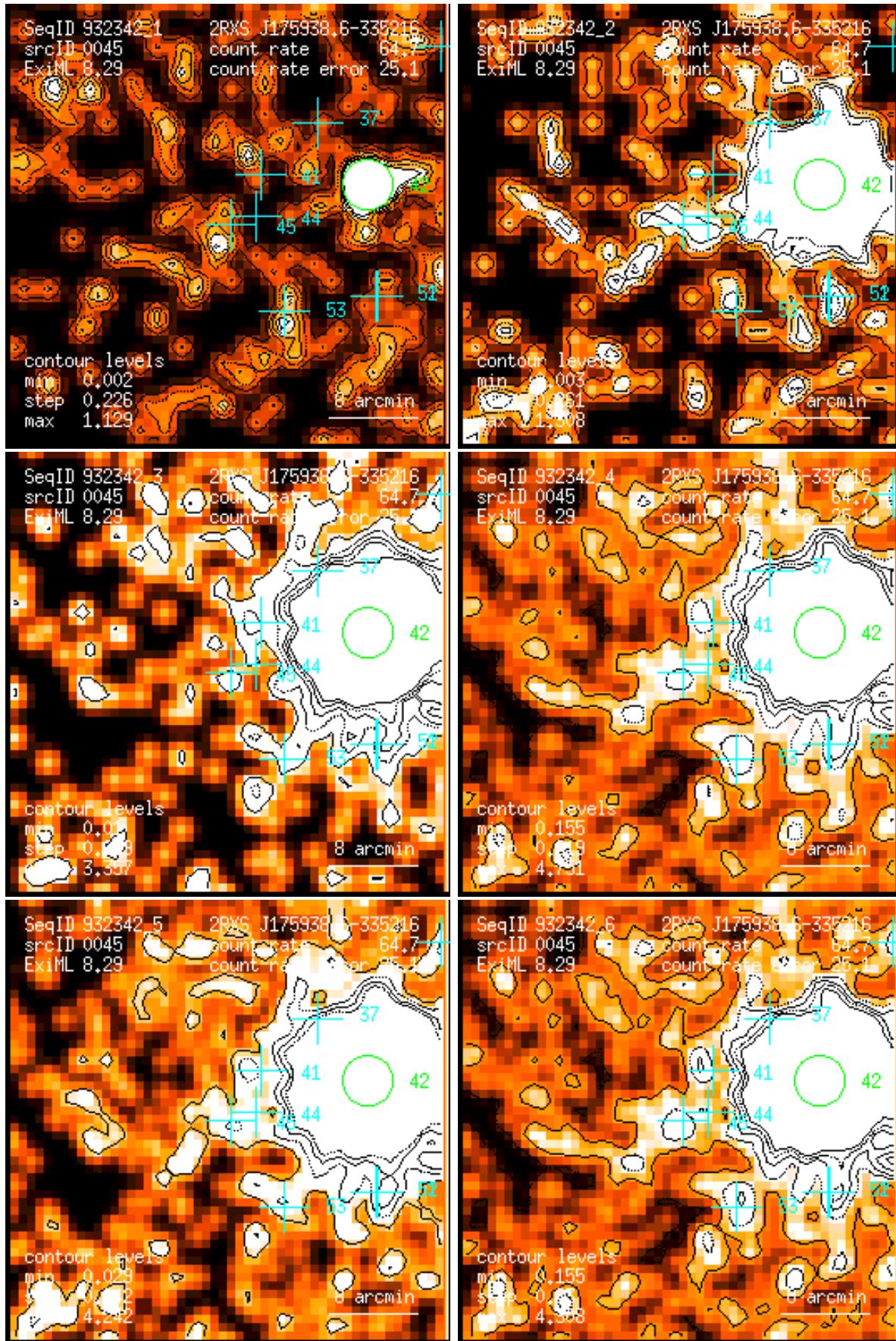
Figure 45: RASS 932342: detection 0045: band rate images, Gaussian filter: (1) PSPC channels 11 – 41, (2) 52 – 90, (3) 91 – 201, (4) 11 – 235, (5) 52 – 201, (6) 11 – 201. Broad band rates in counts/ks. Band rate contour levels in counts/ks/arcmin 2 .
