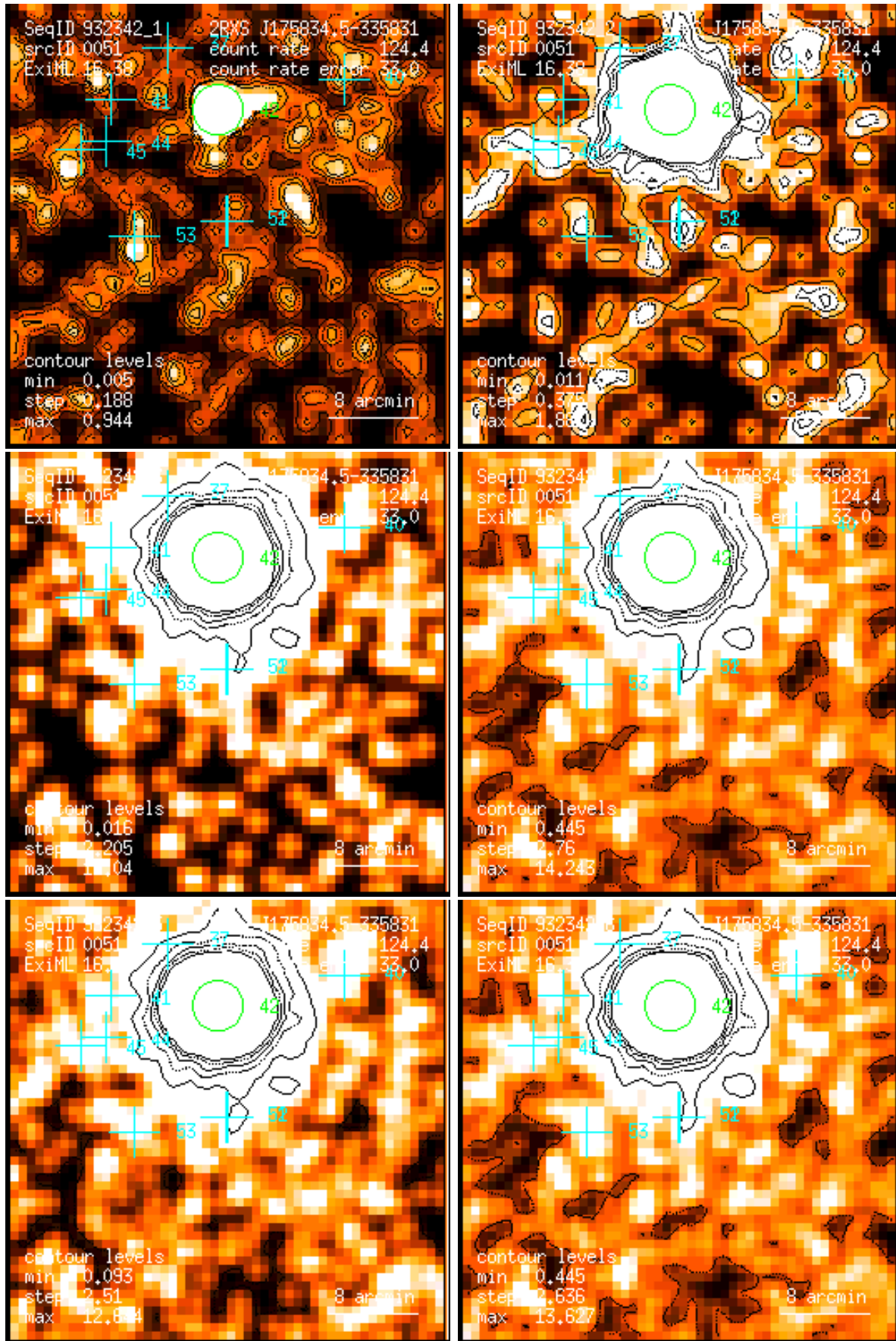
Figure 51: RASS 932342: detection 0051: band rate images, Gaussian filter: (1) PSPC channels 11 – 41, (2) 52 – 90, (3) 91 – 201, (4) 11 – 235, (5) 52 – 201, (6) 11 – 201. Broad band rates in counts/ks. Band rate contour levels in counts/ks/arcmin 2 .
