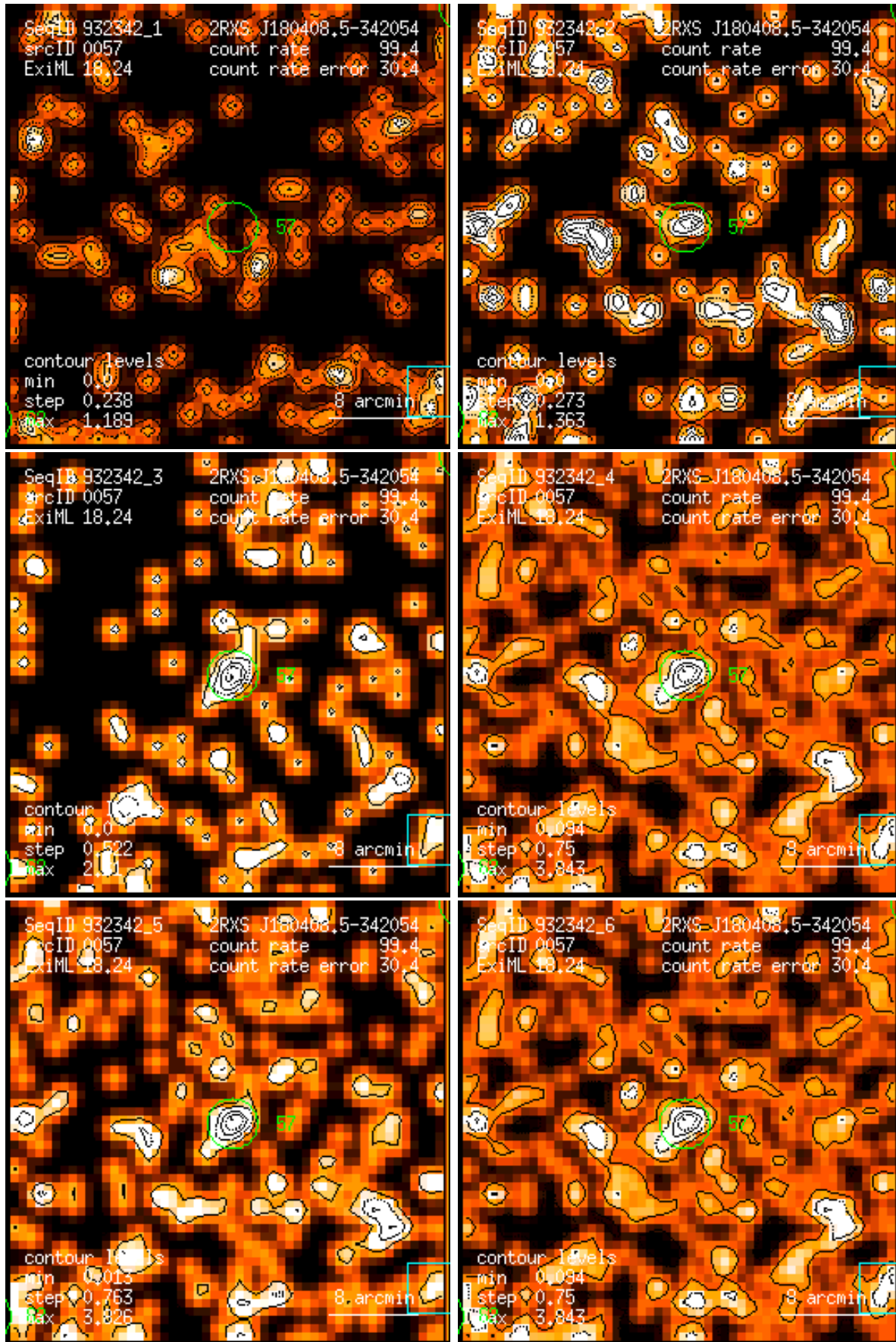
Figure 57: RASS 932342: detection 0057: band rate images, Gaussian filter: (1) PSPC channels 11 – 41, (2) 52 – 90, (3) 91 – 201, (4) 11 – 235, (5) 52 – 201, (6) 11 – 201. Broad band rates in counts/ks. Band rate contour levels in counts/ks/arcmin 2 .
