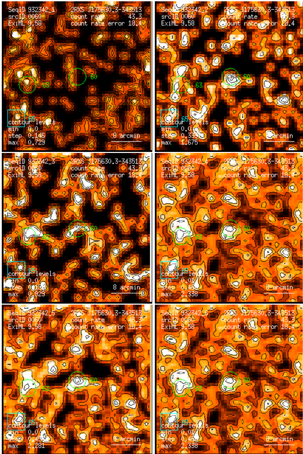
Figure 60: RASS 932342: detection 0060: band rate images, Gaussian filter: (1) PSPC channels 11 – 41, (2) 52 – 90, (3) 91 – 201, (4) 11 – 235, (5) 52 – 201, (6) 11 – 201. Broad band rates in counts/ks. Band rate contour levels in counts/ks/arcmin 2 .
