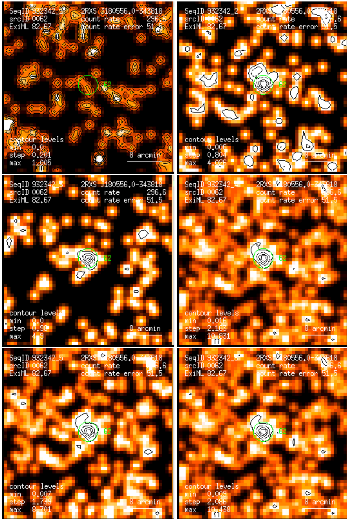
Figure 62: RASS 932342: detection 0062: band rate images, Gaussian filter: (1) PSPC channels 11 – 41, (2) 52 – 90, (3) 91 – 201, (4) 11 – 235, (5) 52 – 201, (6) 11 – 201. Broad band rates in counts/ks. Band rate contour levels in counts/ks/arcmin 2 .
