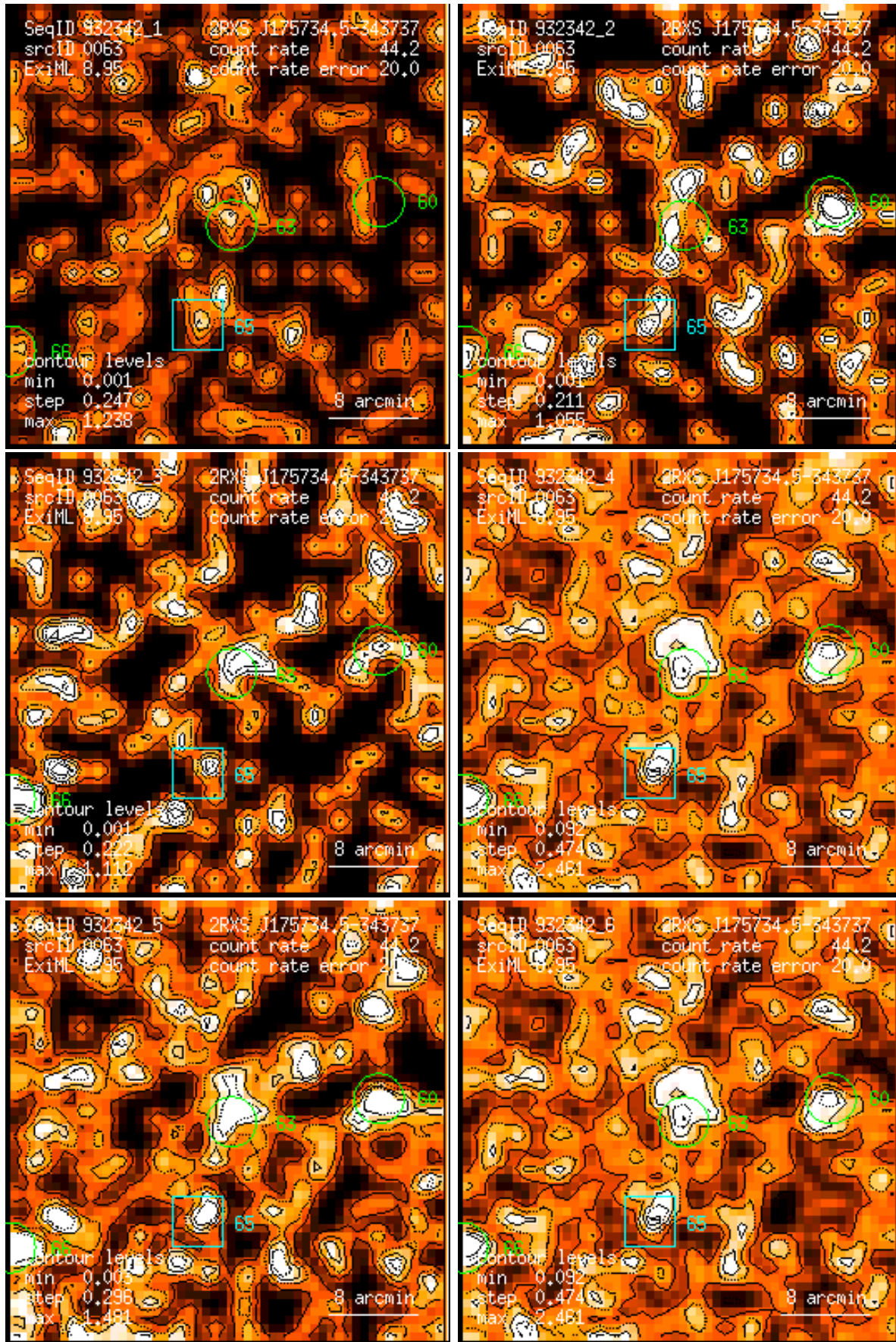
Figure 63: RASS 932342: detection 0063: band rate images, Gaussian filter: (1) PSPC channels 11 – 41, (2) 52 – 90, (3) 91 – 201, (4) 11 – 235, (5) 52 – 201, (6) 11 – 201. Broad band rates in counts/ks. Band rate contour levels in counts/ks/arcmin 2 .
