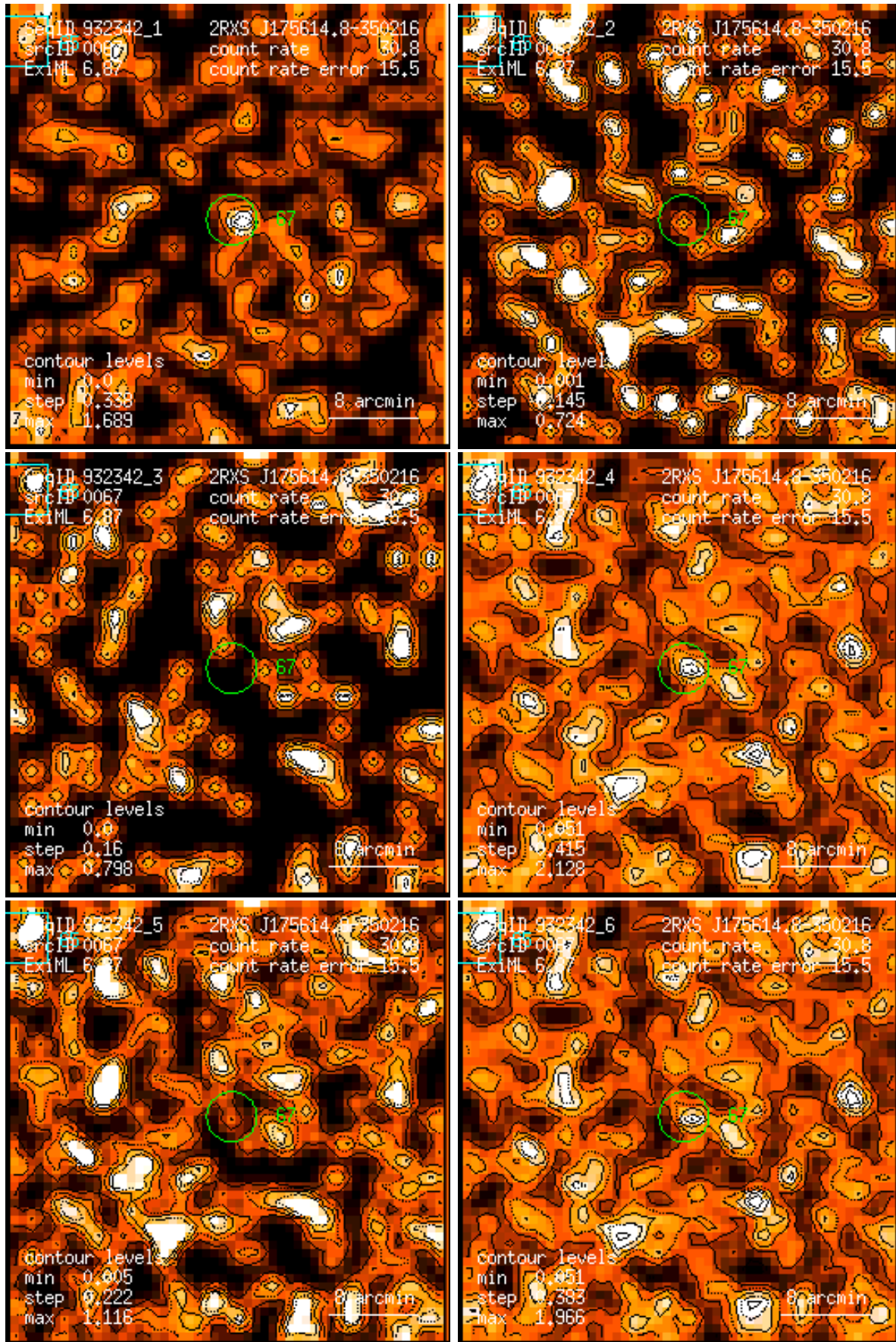
Figure 67: RASS 932342: detection 0067: band rate images, Gaussian filter: (1) PSPC channels 11 – 41, (2) 52 – 90, (3) 91 – 201, (4) 11 – 235, (5) 52 – 201, (6) 11 – 201. Broad band rates in counts/ks. Band rate contour levels in counts/ks/arcmin 2 .
