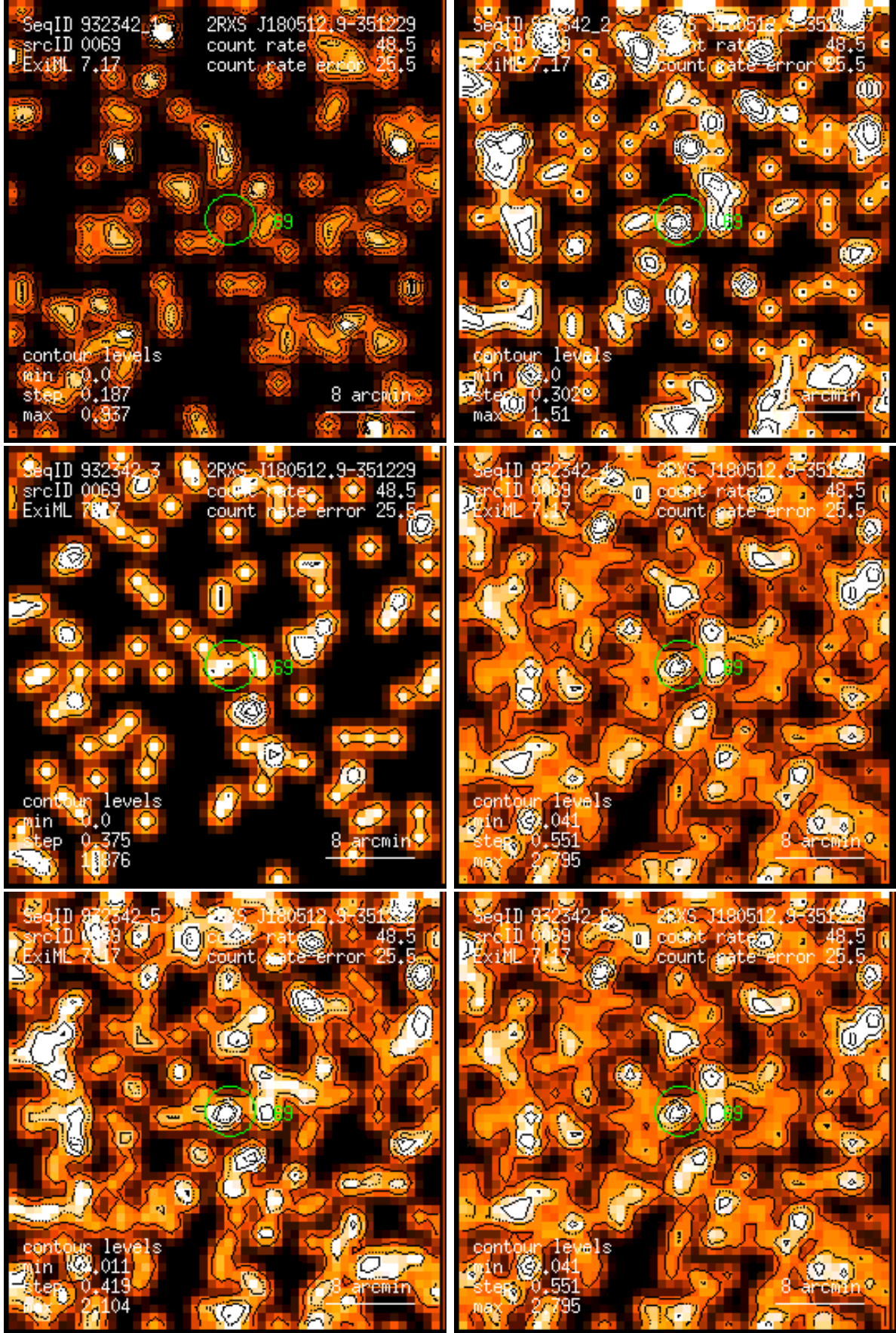
Figure 69: RASS 932342: detection 0069: band rate images, Gaussian filter: (1) PSPC channels 11 – 41, (2) 52 – 90, (3) 91 – 201, (4) 11 – 235, (5) 52 – 201, (6) 11 – 201. Broad band rates in counts/ks. Band rate contour levels in counts/ks/arcmin 2 .
