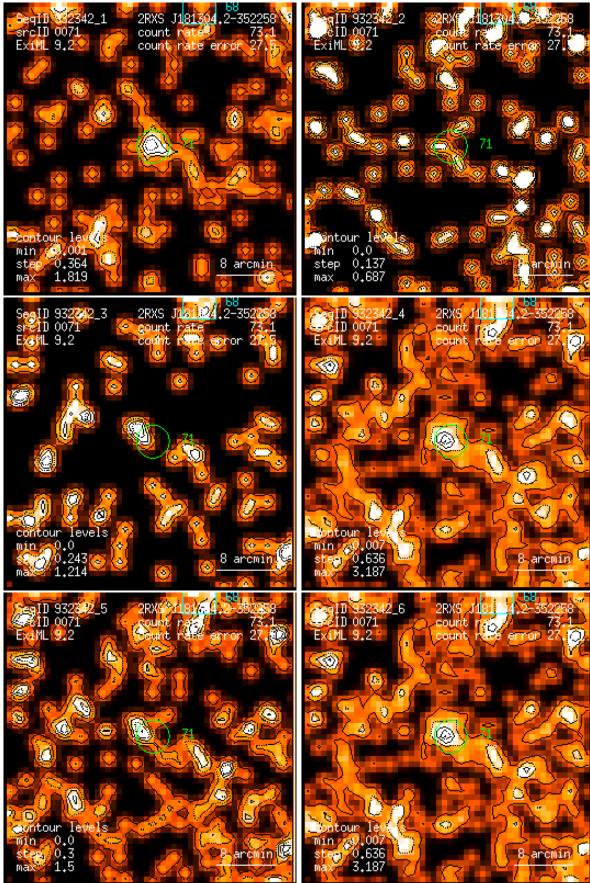
Figure 71: RASS 932342: detection 0071: band rate images, Gaussian filter: (1) PSPC channels 11 – 41, (2) 52 – 90, (3) 91 – 201, (4) 11 – 235, (5) 52 – 201, (6) 11 – 201. Broad band rates in counts/ks. Band rate contour levels in counts/ks/arcmin 2 .
