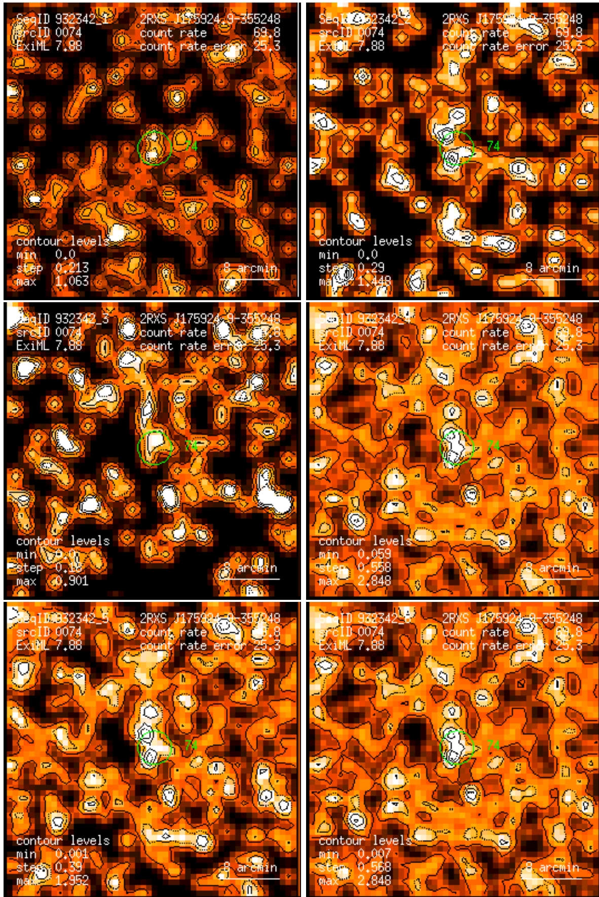
Figure 74: RASS 932342: detection 0074: band rate images, Gaussian filter: (1) PSPC channels 11 – 41, (2) 52 – 90, (3) 91 – 201, (4) 11 – 235, (5) 52 – 201, (6) 11 – 201. Broad band rates in counts/ks. Band rate contour levels in counts/ks/arcmin 2 .
