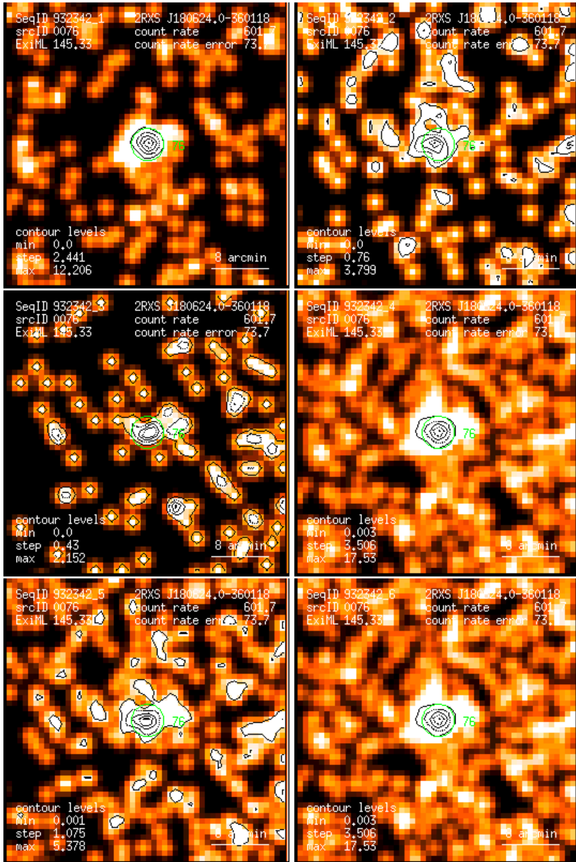
Figure 76: RASS 932342: detection 0076: band rate images, Gaussian filter: (1) PSPC channels 11 – 41, (2) 52 – 90, (3) 91 – 201, (4) 11 – 235, (5) 52 – 201, (6) 11 – 201. Broad band rates in counts/ks. Band rate contour levels in counts/ks/arcmin 2 .
