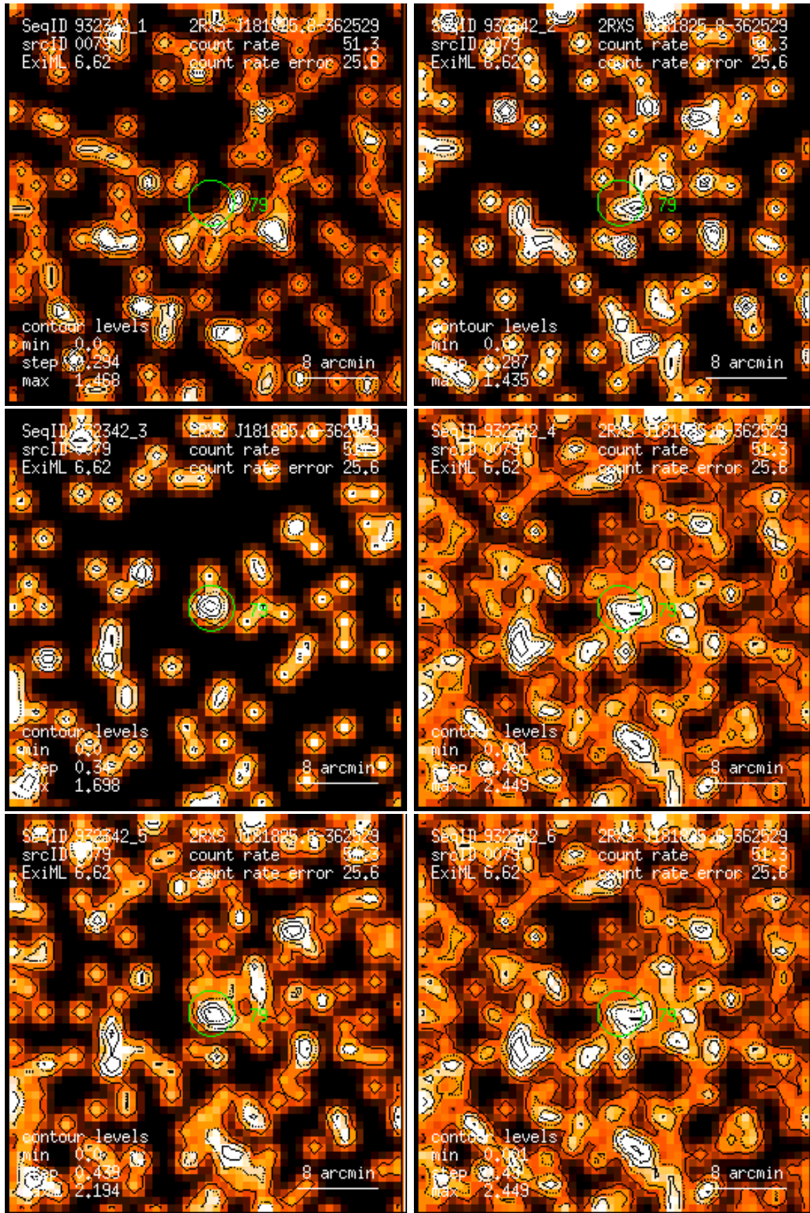
Figure 79: RASS 932342: detection 0079: band rate images, Gaussian filter: (1) PSPC channels 11 – 41, (2) 52 – 90, (3) 91 – 201, (4) 11 – 235, (5) 52 – 201, (6) 11 – 201. Broad band rates in counts/ks. Band rate contour levels in counts/ks/arcmin 2 .
