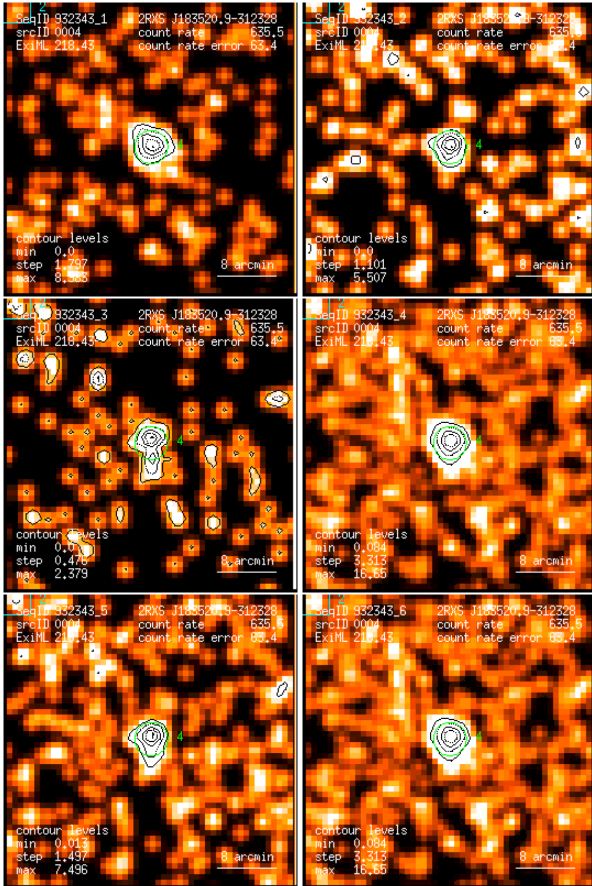
Figure 4: RASS 932343: detection 0004: band rate images, Gaussian filter: (1) PSPC channels 11 – 41, (2) 52 – 90, (3) 91 – 201, (4) 11 – 235, (5) 52 – 201, (6) 11 – 201. Broad band rates in counts/ks. Band rate contour levels in counts/ks/arcmin 2 .
