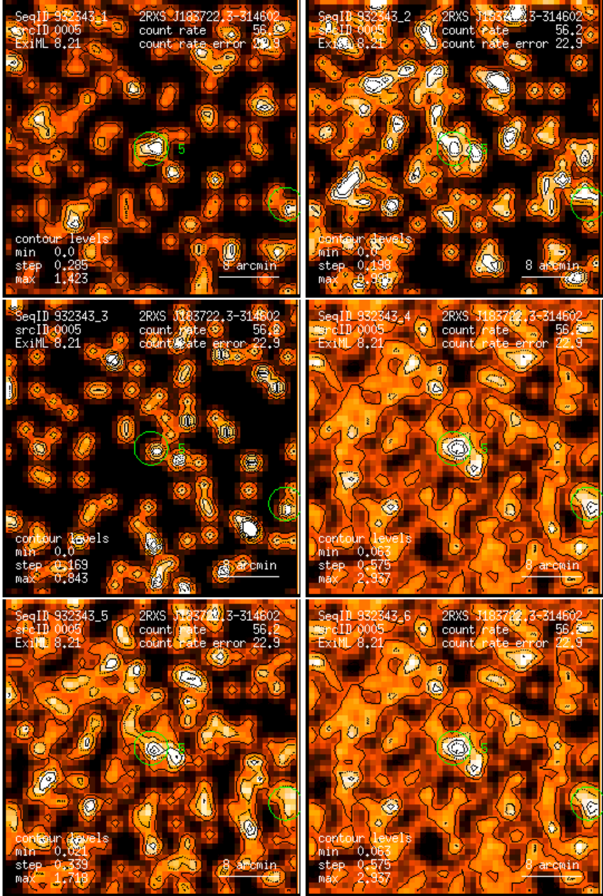
Figure 5: RASS 932343: detection 0005: band rate images, Gaussian filter: (1) PSPC channels 11 – 41, (2) 52 – 90, (3) 91 – 201, (4) 11 – 235, (5) 52 – 201, (6) 11 – 201. Broad band rates in counts/ks. Band rate contour levels in counts/ks/arcmin 2 .
