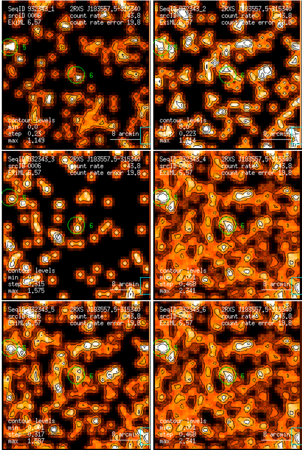
Figure 6: RASS 932343: detection 0006: band rate images, Gaussian filter: (1) PSPC channels 11 – 41, (2) 52 – 90, (3) 91 – 201, (4) 11 – 235, (5) 52 – 201, (6) 11 – 201. Broad band rates in counts/ks. Band rate contour levels in counts/ks/arcmin 2 .
