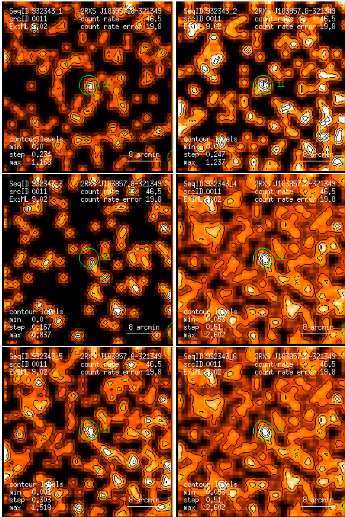
Figure 11: RASS 932343: detection 0011: band rate images, Gaussian filter: (1) PSPC channels 11 – 41, (2) 52 – 90, (3) 91 – 201, (4) 11 – 235, (5) 52 – 201, (6) 11 – 201. Broad band rates in counts/ks. Band rate contour levels in counts/ks/arcmin 2 .
