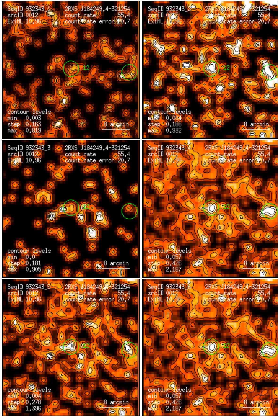
Figure 12: RASS 932343: detection 0012: band rate images, Gaussian filter: (1) PSPC channels 11 – 41, (2) 52 – 90, (3) 91 – 201, (4) 11 – 235, (5) 52 – 201, (6) 11 – 201. Broad band rates in counts/ks. Band rate contour levels in counts/ks/arcmin 2 .
